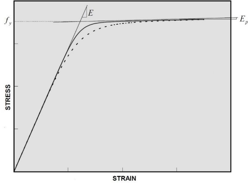
Figure 3.6: Material Parameters for Steel model.
