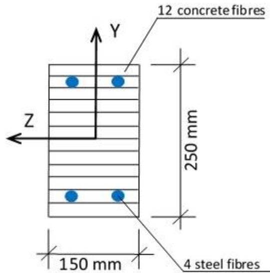
Figure 4.15: Fibre beam element cross section mesh for sample S1616-A and S1616-D.
