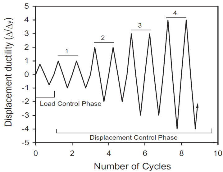
Figure 3.35: loading history, Figure from Caballero-Morrison et al. (2013) .
