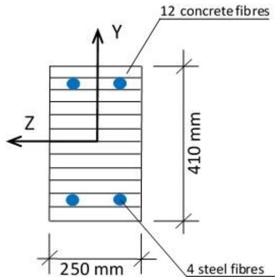
Figure 4.9: Fibre beam element cross section mesh for sample SS3a-1.
