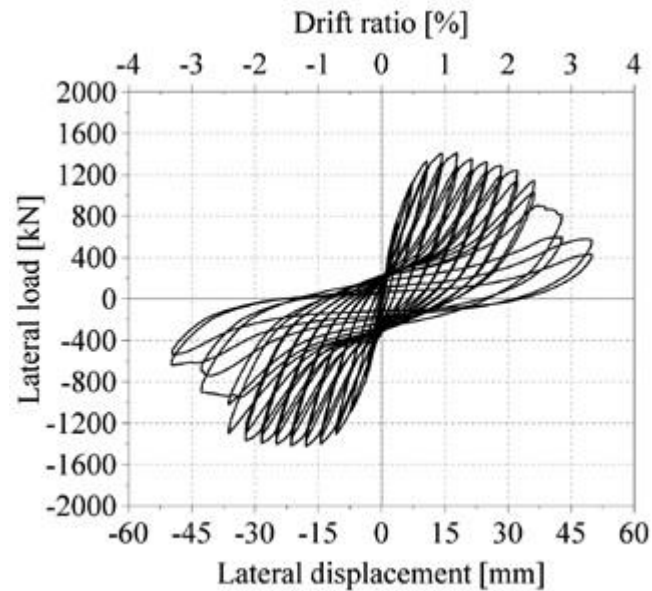
Figure 5.11: Experimental load-displacement relationships for SC1, Figure from Epackachi et al. (2015) .
