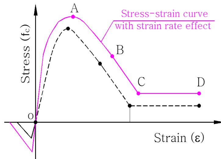
Figure 4.5: Concrete material model with and without strain rate effect.
