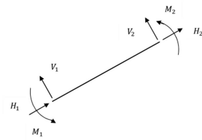
Figure 3.2: Internal element loading with respect to corotational system.
