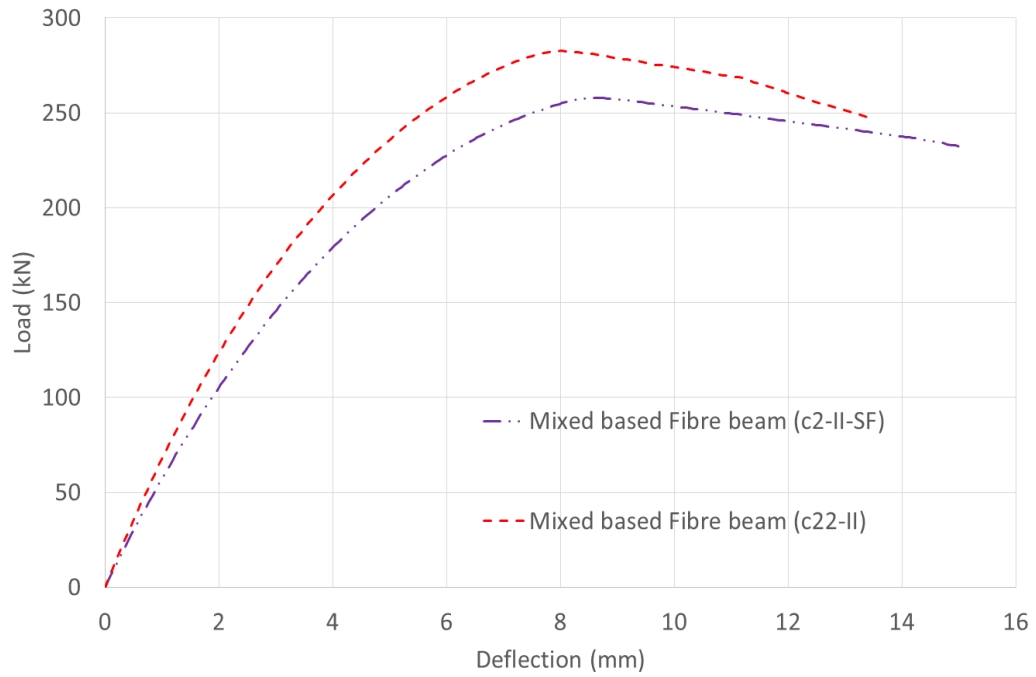
Figure 3.53: Load-deflection curve for columns C2-II & C2-II-SF using the mixed fibre beam element.
