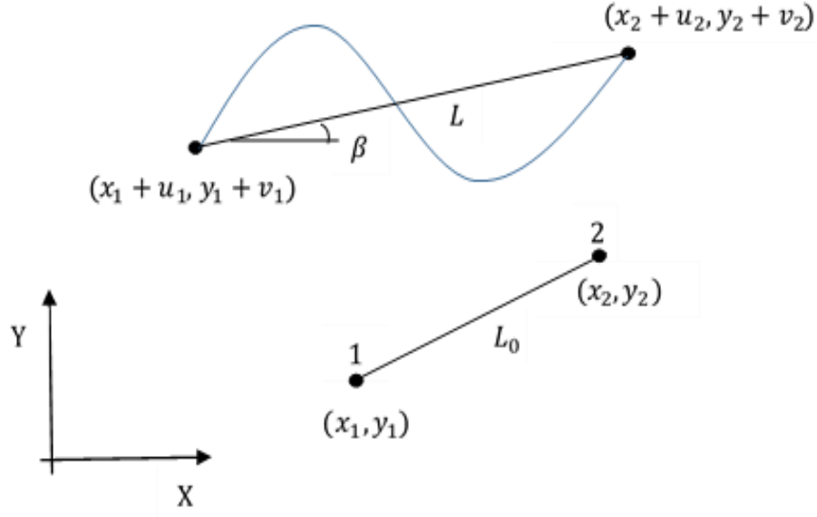
Figure 3.3: Initial state and final element configuration.
