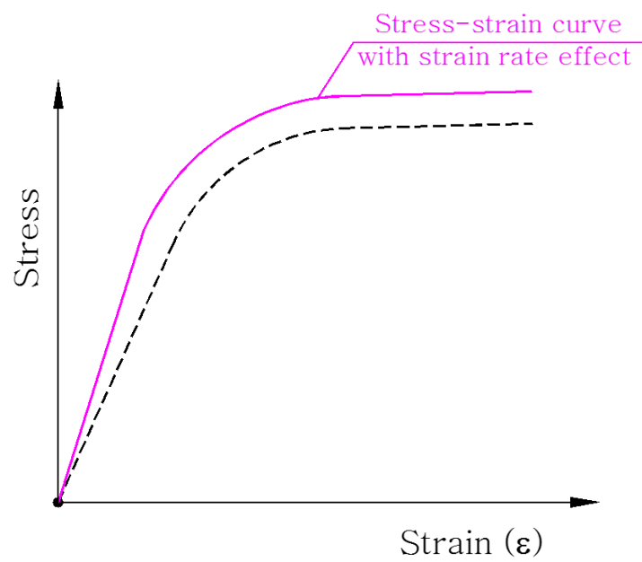
Figure 4.6: Menegotto-Pinto monotonic stress-strain curve of mild steel bar with and without strain rate effect.
