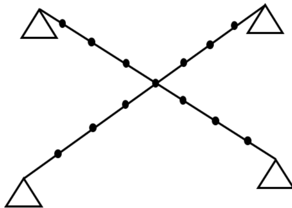
Figure 5.20: Fibre beam element 2D model (1 row/direction).
