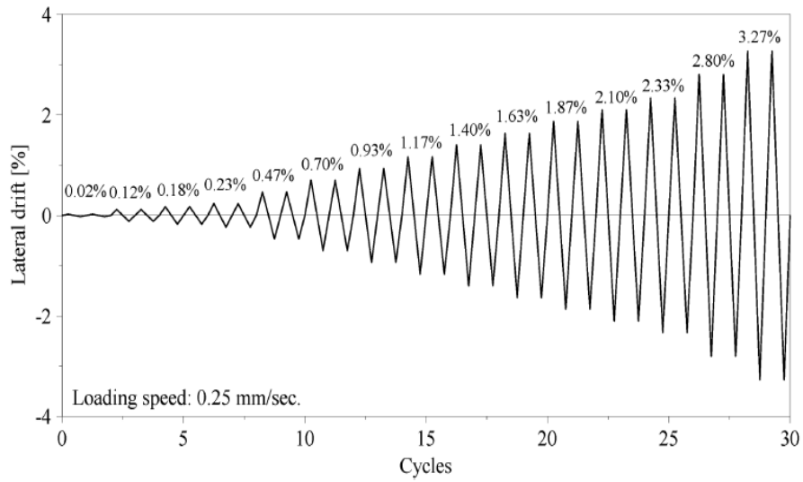
Figure 5.8: Loading protocol, Figure from Epachachi et al. (2015) .
