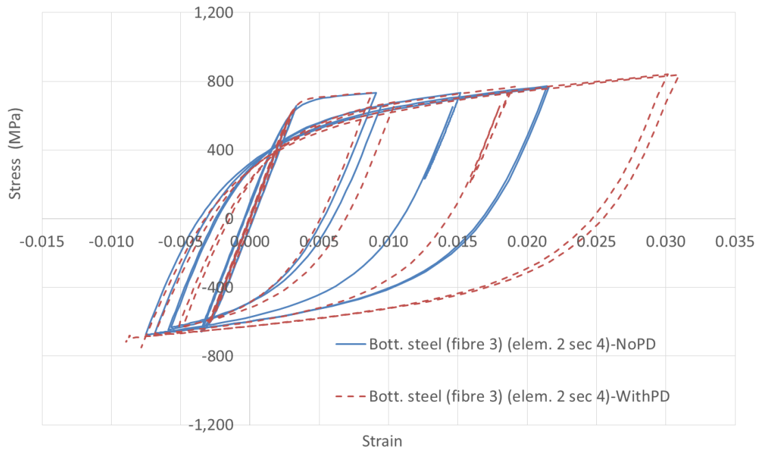
Figure 3.46: Comparison between the stress strain curves of bottom steel fibre 3 for element 2 at sec 4 using the mixed element with and without the second order effect (sample HF60L05V1S50).
