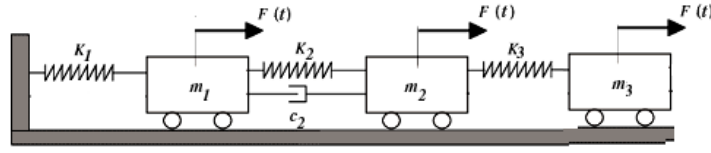
Figure (8.57): The open-loop system of Example (8.7)
