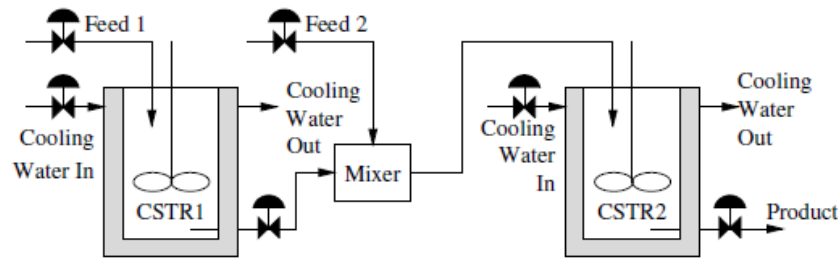
Figure (5.12): Two-CSTR Process
