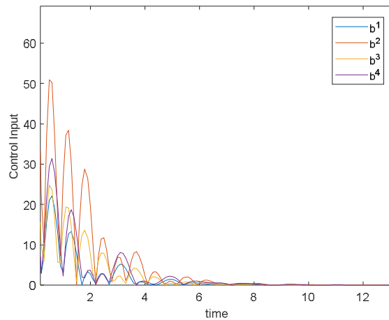
Figure (8.62): Control force input needed to control the system when using the input vector
