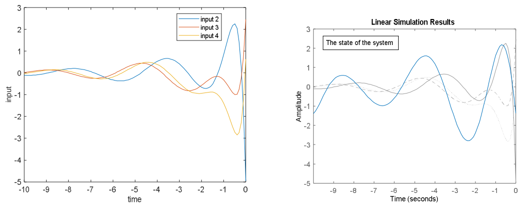
Figure (8.55): The input and state of the system with the actuator set s_{actuator} = \{2, 3, 4\}
