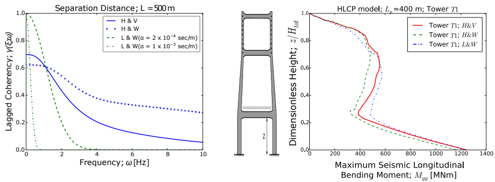
Fig. 3. (a) Comparison of the different coherency models. (b) Peak longitudinal, M_{yy} , bending moment along the tower of the bridge with L_p = 400\text{m} for different coherency models.
