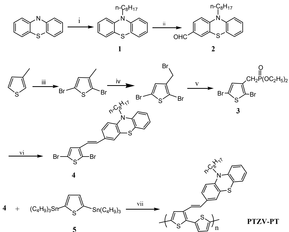
Scheme 2. Synthetic route of the monomers and polymer PTZV-PT
