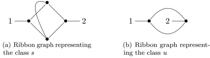
FIGURE 4. Ribbon graphs corresponding to generators of \pi_0(M_*)
