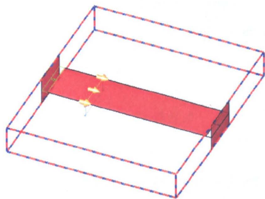
Figure 3.20. Stripline structure with 50 \, \Omega characteristic impedance.
