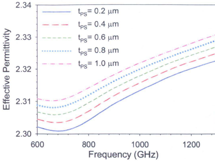
Figure 4.28. Effective permittivity of the microstrip structure for different values of polystyrene thickness (0 – 1.0 \mu m ).
