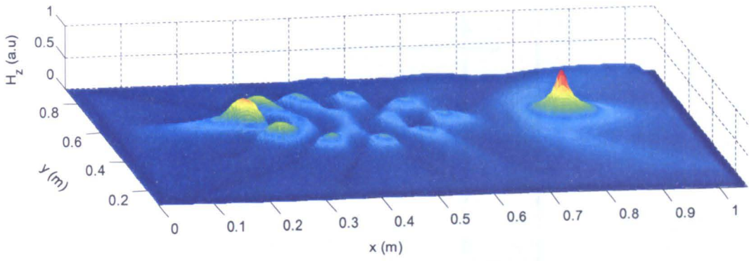
Figure 3.17. Magnetic field distribution sampled at 1 GHz.
