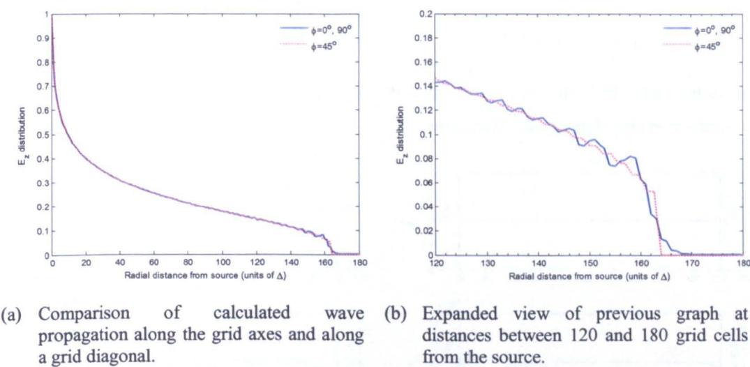
Figure 3.10. Effect of numerical dispersion in a two-dimensional grid upon a radially propagating cylindrical wave.
