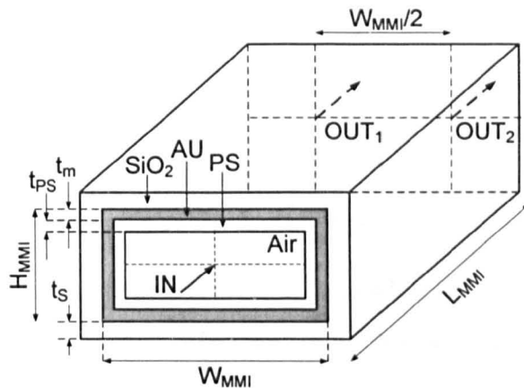
Figure 5.2. Hollow-core polystyrene coated Terahertz Multimode Interference device.
