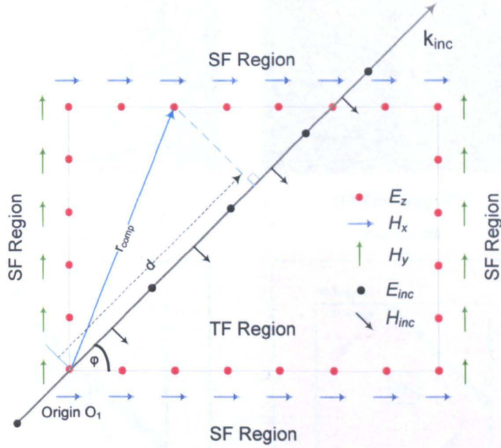
Figure 3.26. Incident plane-wave calculation for the 2D TF/SF FDTD formulation ( \text{TM}_z ).
