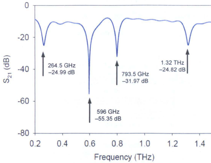
Figure 4.11. Transmission parameters of the microstrip/filter array.
