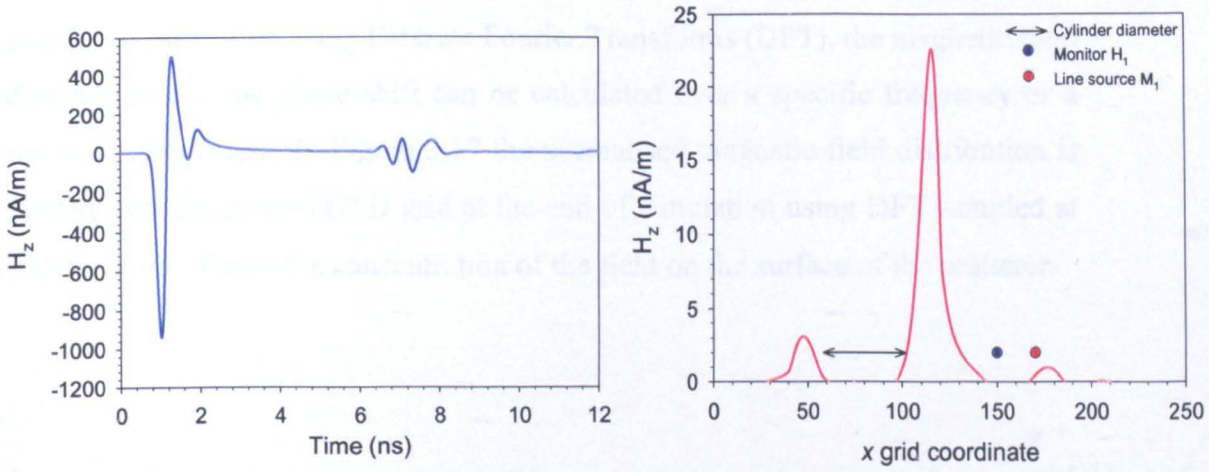
(a) Sampled magnetic field H_z at monitor H_1 . (b) Magnetic field H_z along the propagation direction
