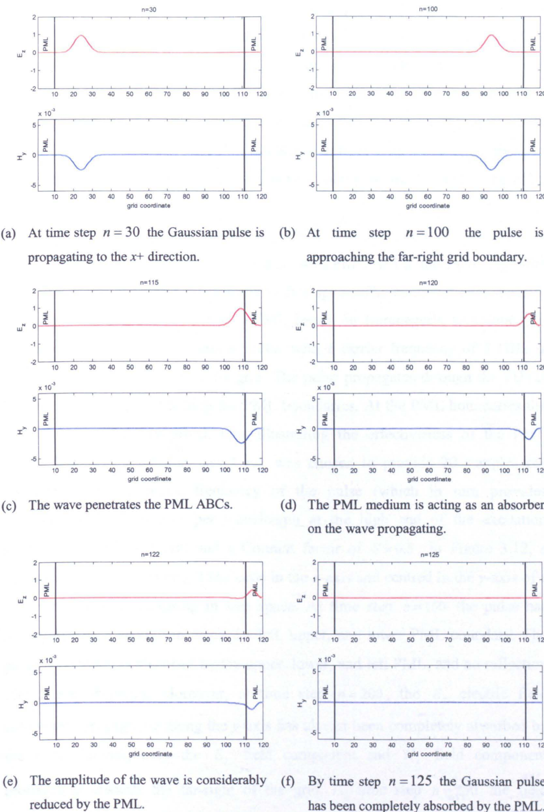
Figure 3.11. One-dimensional plane wave propagation with PML ABCs.
