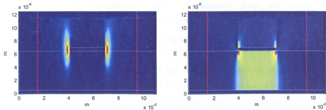
(a) Sampled electric field E_x at 1 THz for the microstrip line with no PS coating.
