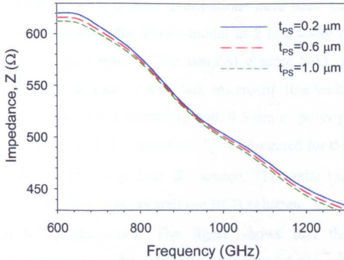
Figure 4.29. Characteristic impedance of the microstrip structure for different values of polystyrene thickness (0 – 1.0 \mu m ).
