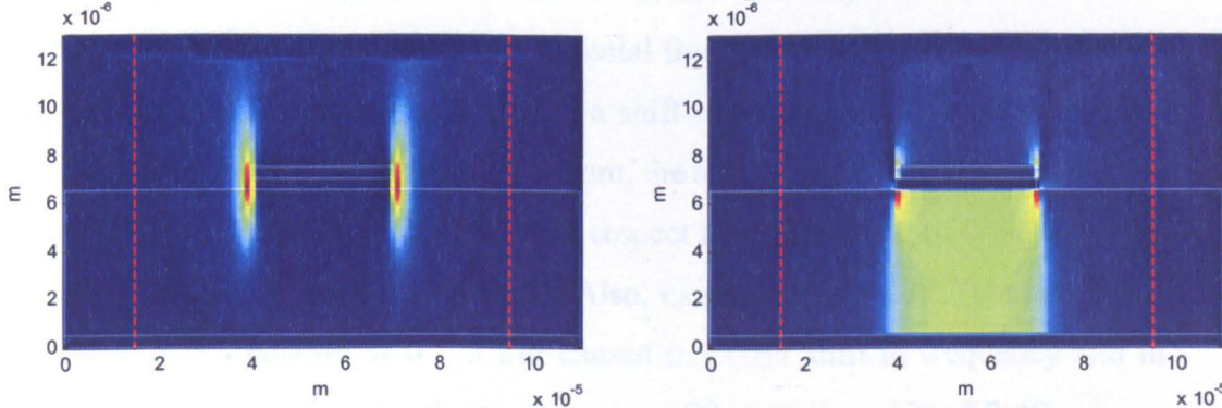
(c) Sampled electric field E_x at 1 THz for the microstrip line with 0.5 \mu\text{m} PS coating.
