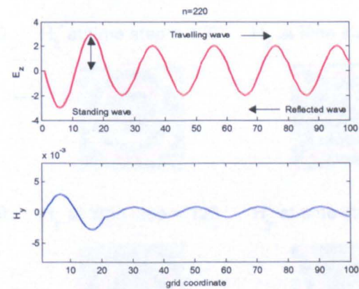
(f) Retro-reflection effect, a new standing wave at time-step n = 220 .
