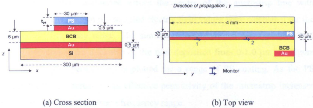
Figure 4.27. Microstrip with PS coating (not to scale).
