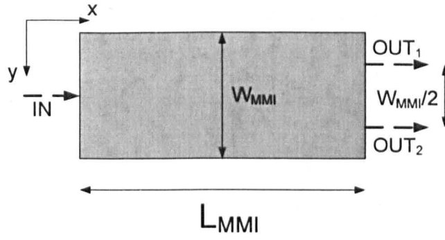
Figure 5.4. MMI device layout.
