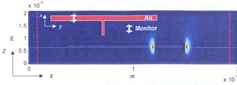
(a) Sampled electric field E_x at 1 THz for the microstrip line.
