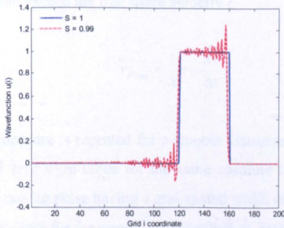
Figure 2.9. Rectangular pulse propagation for S = 1 and S = 0.99 .
