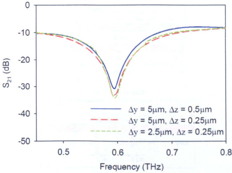
Figure 4.9. Insertion loss and effective permittivity of microstrip line for different FDTD cell parameters for \Delta x = 1\text{ }\mu\text{m} .
