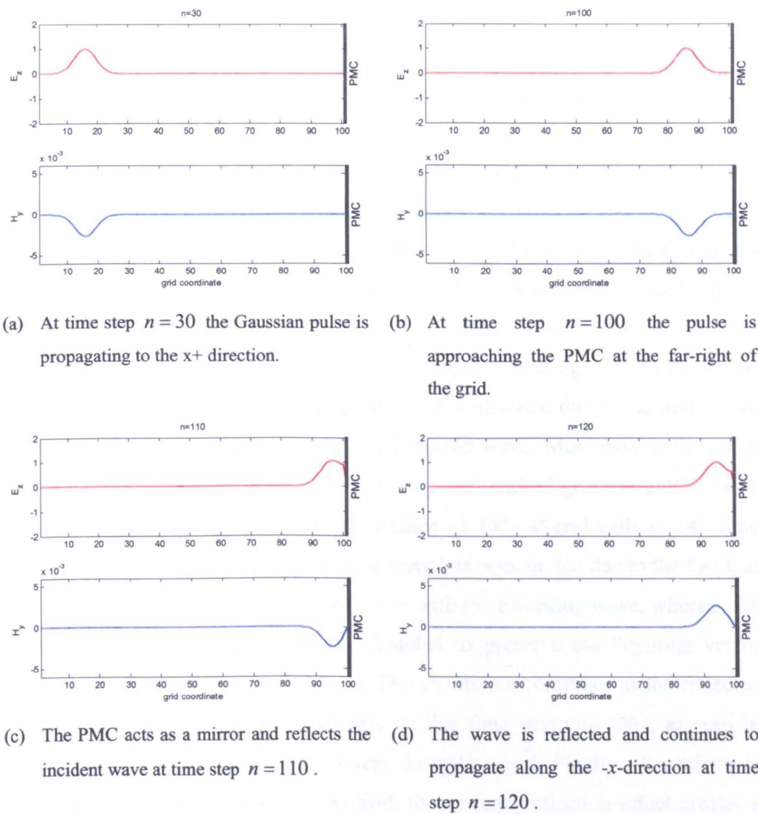
Figure 3.2. One-dimensional plane wave propagation with PMC boundary.
