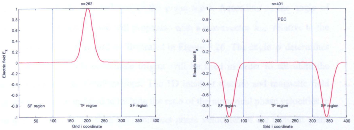
(a) Gaussian pulse propagating in free-space.
