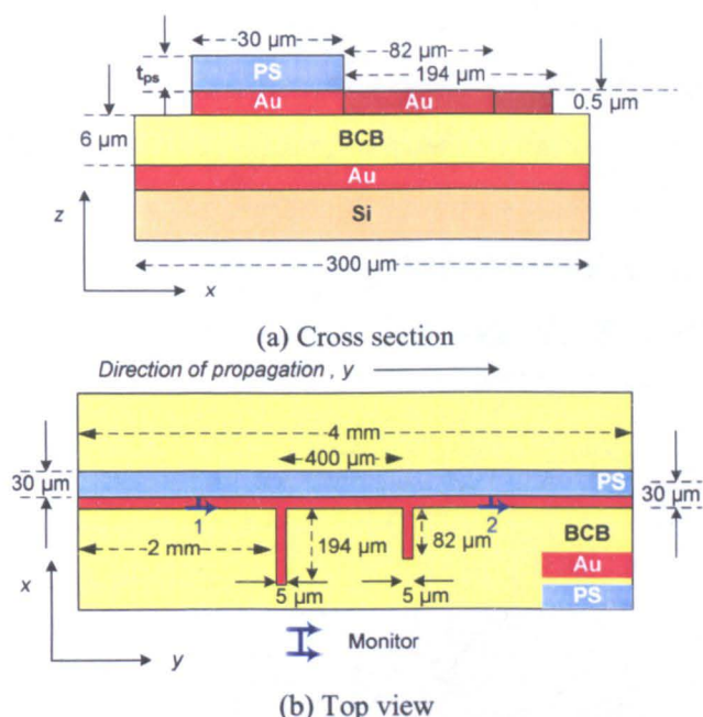
Figure 4.18. Geometry of the microstrip structure, filters, and polystyrene coating (not to scale).
