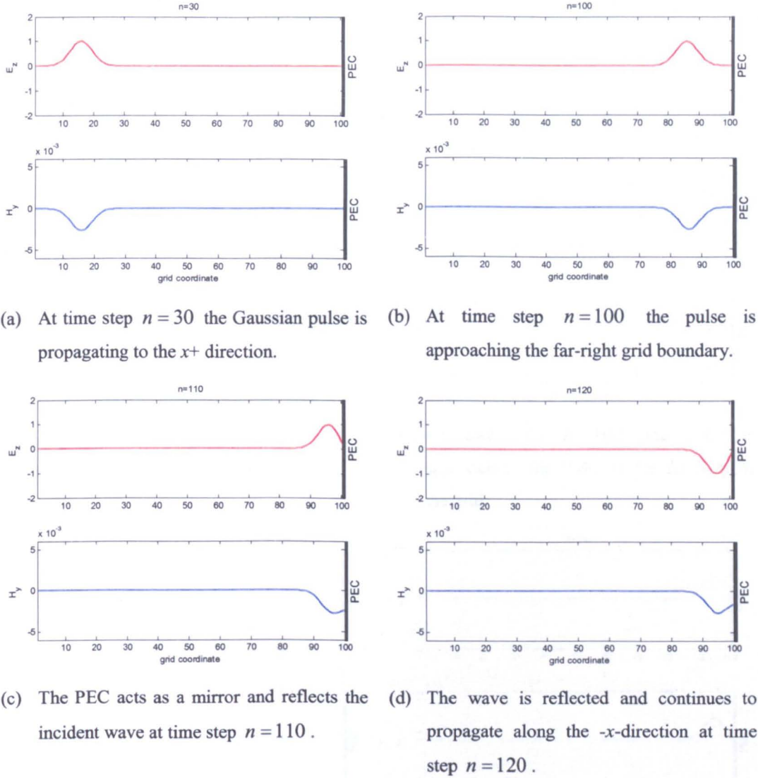
Figure 3.1. One-dimensional plane wave propagation with PEC boundary.
