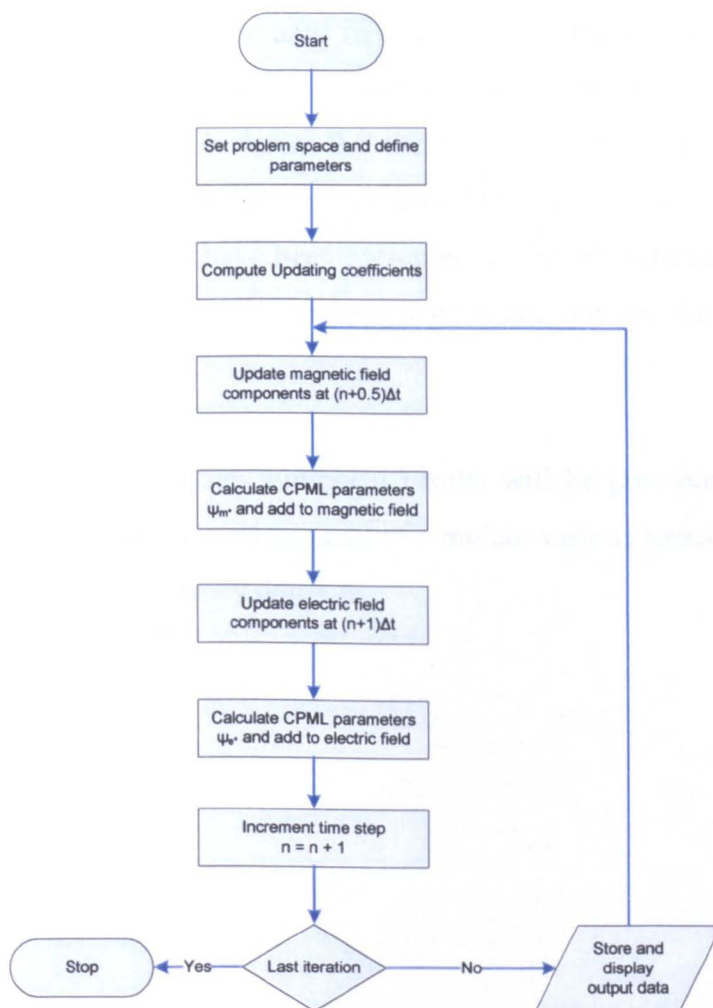
Figure 2.19. The FDTD algorithm including the CPML steps.
