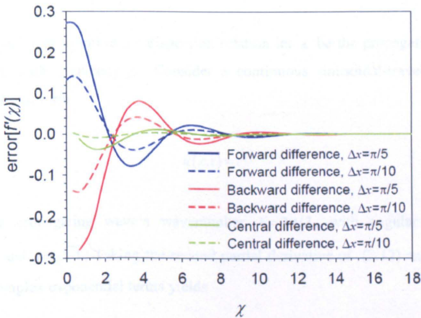
Figure 2.5. Finite differences formulae error calculated for \Delta x = \pi/5 and \Delta x = \pi/10 sampling rates.
