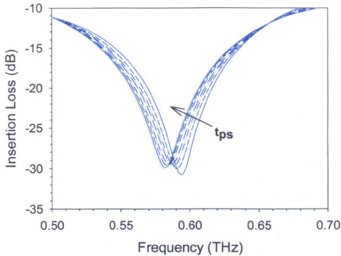
Figure 4.15. Insertion loss of the microstrip structure for different values of polystyrene thickness (0 – 15 \mu\text{m} ) with single filter.
