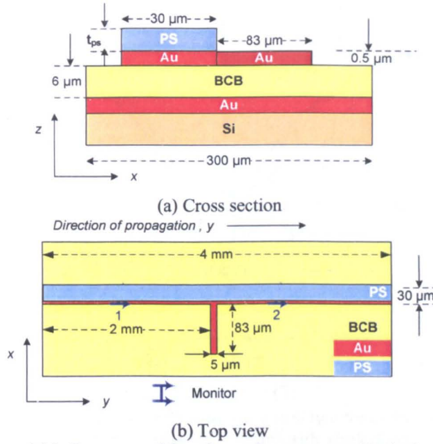
Figure 4.14. Geometry of the microstrip structure with single filter, and polystyrene coating (not to scale).
