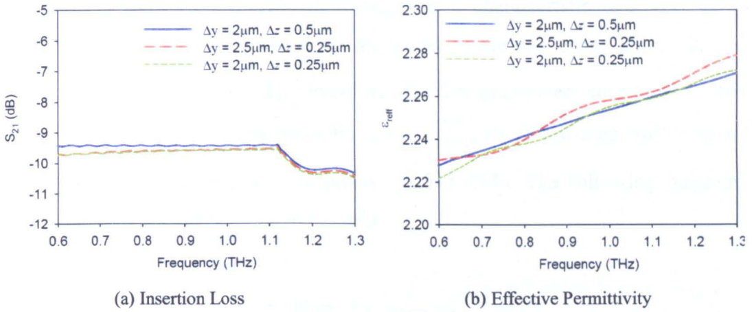
Figure 4.5. Insertion loss and effective permittivity of microstrip line for different FDTD cell parameters for \Delta x = 1 \mu m .
