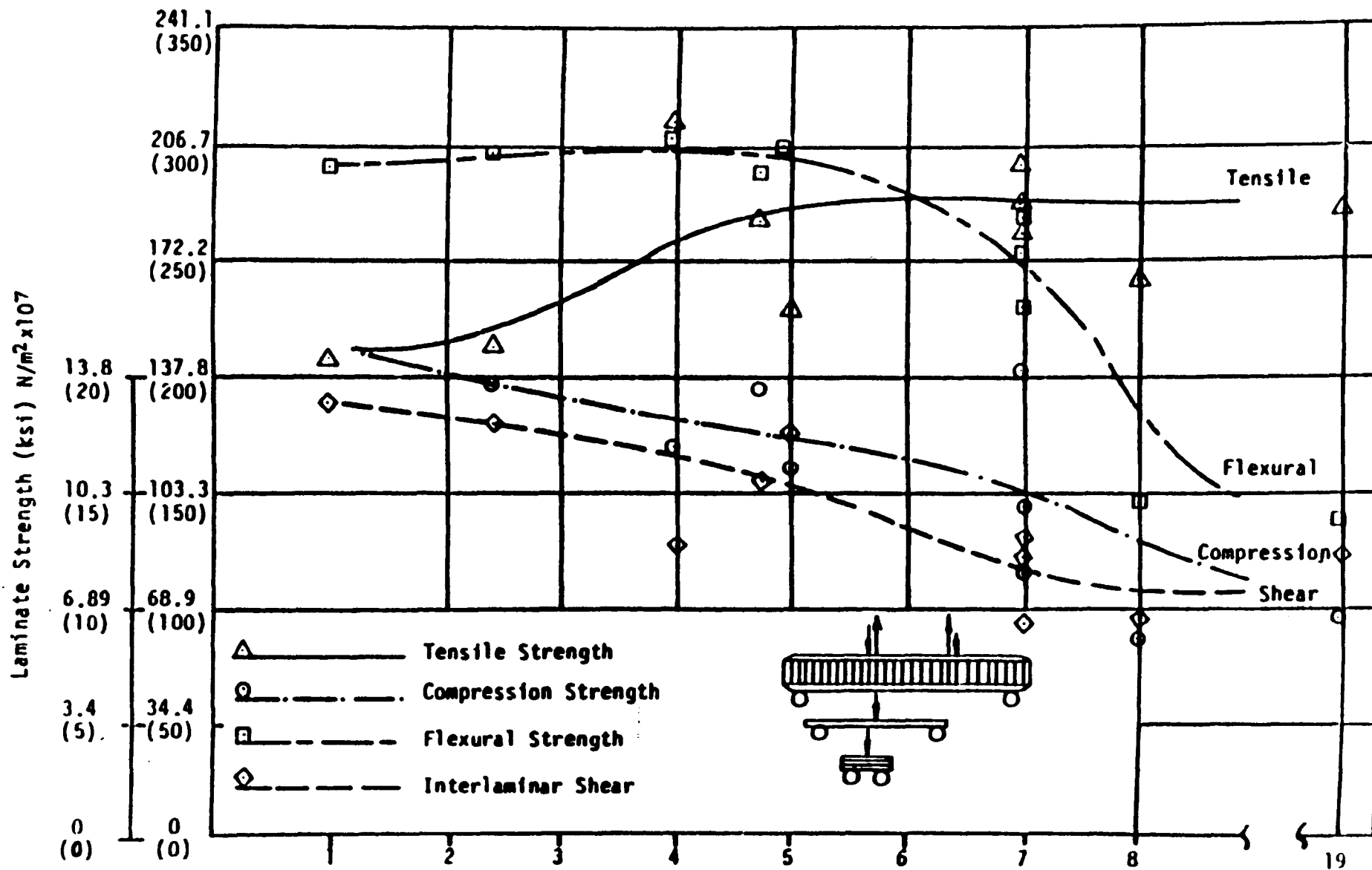
FIGURE 6. RESIN TENSILE ELONGATION VS LAMINATE MECHANICAL PROPERTIES
