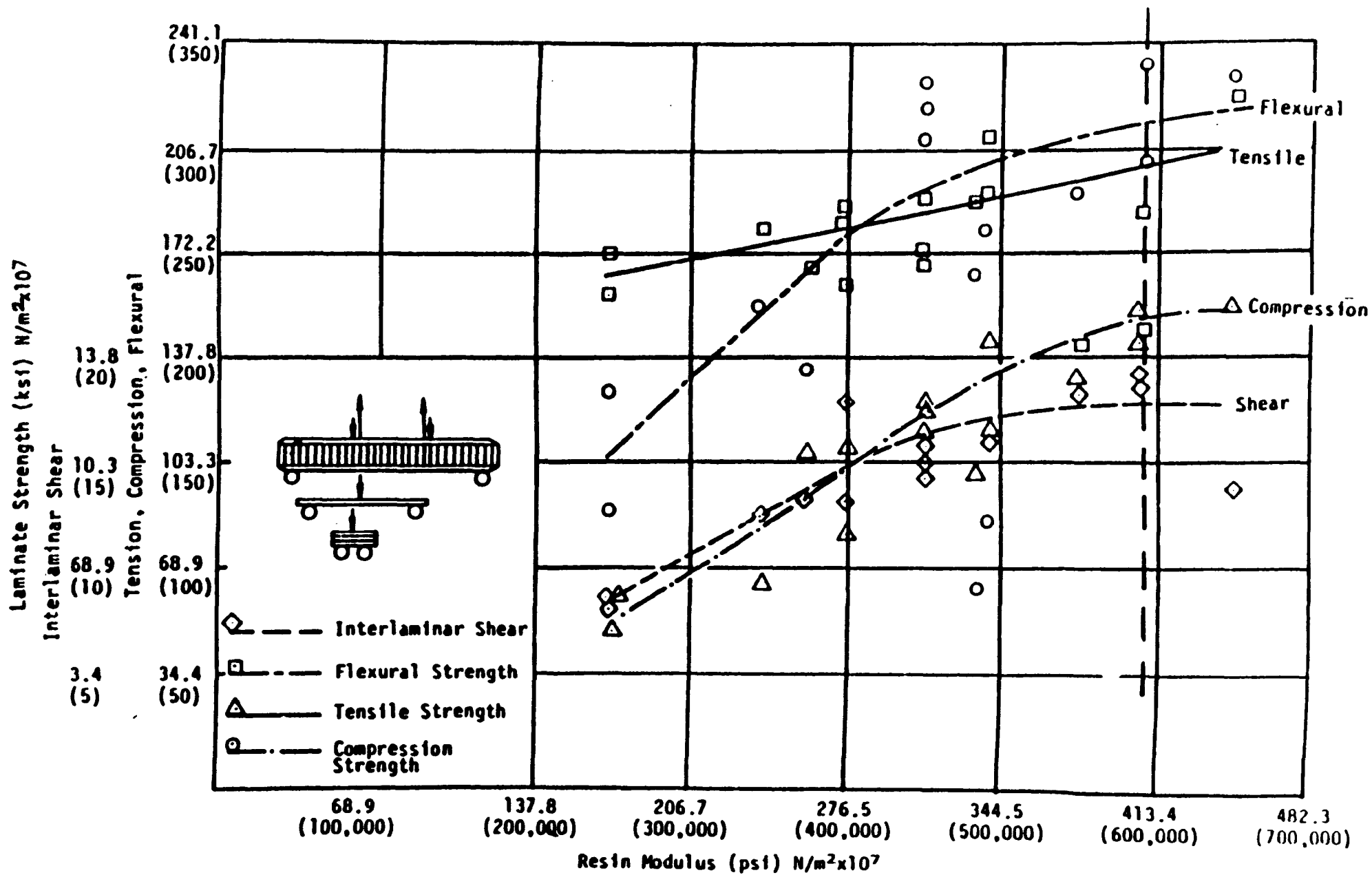
FIGURE 5. RESIN TENSILE MODULUS VS LAMINATE MECHANICAL PROPERTIES
