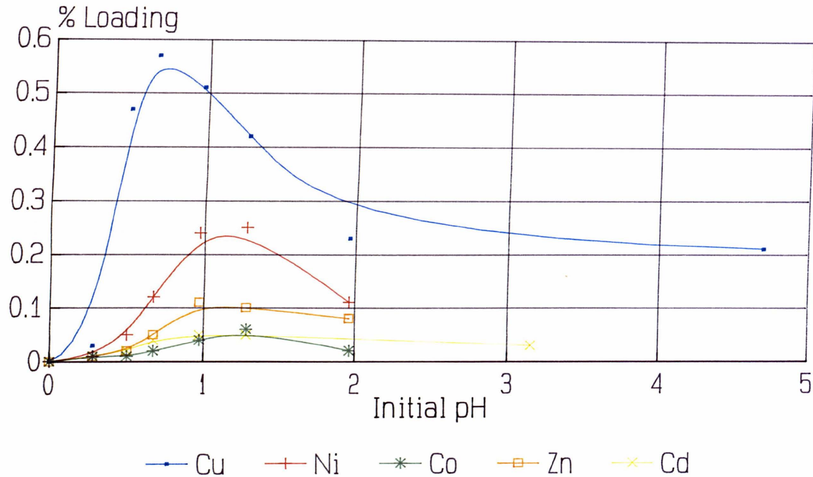
Figure 4.1 Effect Of Initial pH On Loading
