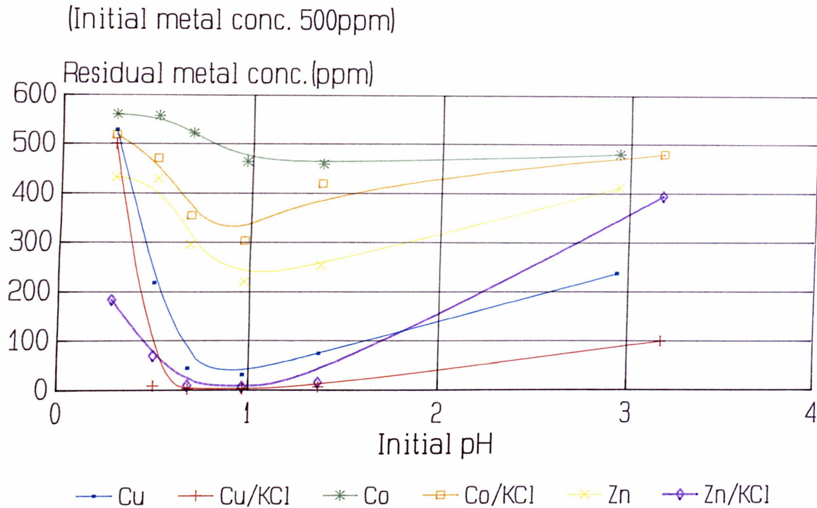
Figure 4.6 Effect Of pH On Purification Of 40g/l KCl And Dilute Solutions
