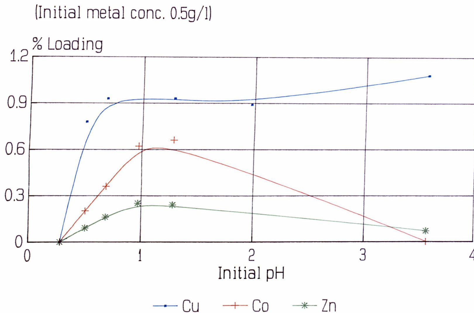
Figure 4.4 Effect Of High Chloride Conc. On Loading
