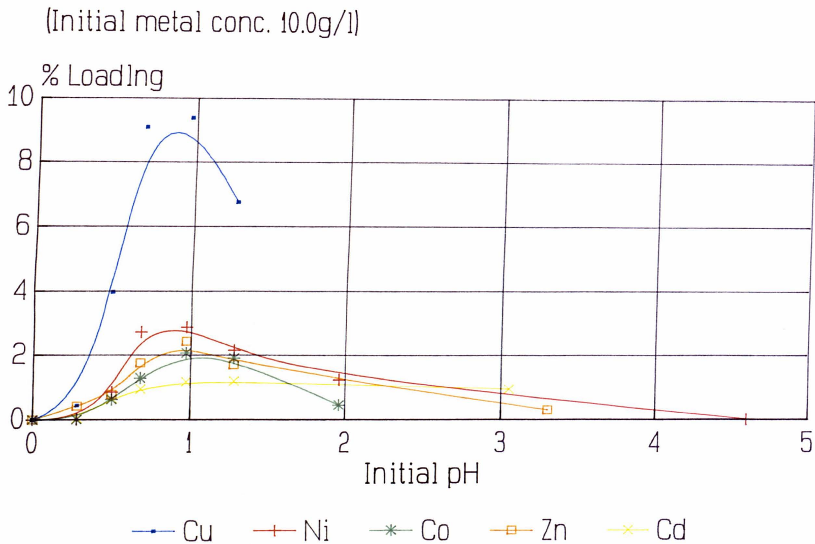
Figure 4.2 Effect Of Initial pH On Loading
