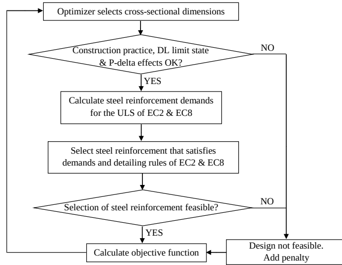
Fig. 2: Optimum seismic design to EC8 flowchart
