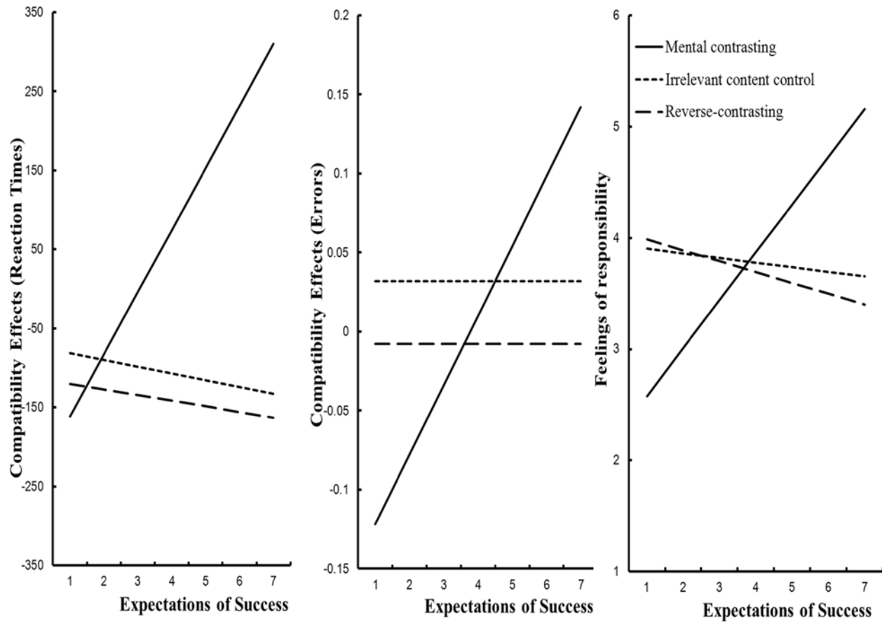
Figure 2. Study 2: Regression lines depict the relations between expectations of success and compatibility effects derived from reaction times (left), compatibility effects derived from errors (middle), and feelings of responsibility (right) as a function of condition.
