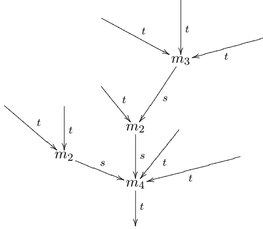
FIGURE 1. Definition of \tilde{m}_T .
