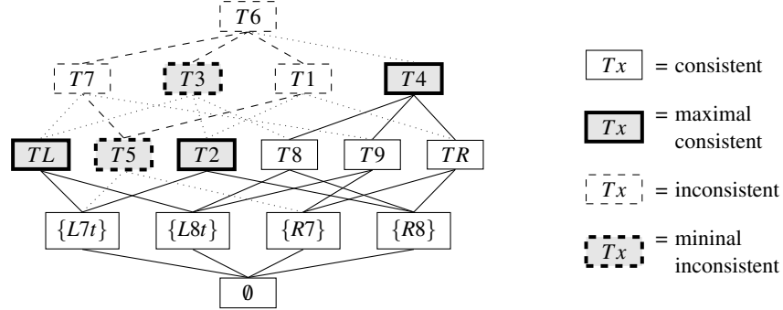
Fig. 4. A lattice of the ‘blends’ that appear in the given example.
