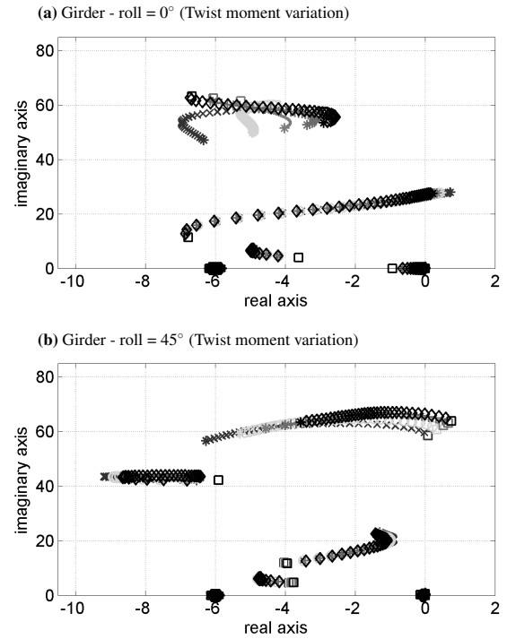
Fig. 23: Root loci for the Girder suspension system with constant normal trail ( cnt ) configuration. The twist moment coefficients are varied as 60% (blue \times ), 80% (green \circ ), 100% (magenta \cdot ), 120% (red + ) and 140% (black \diamond ) of the nominal value. The speed is increased from 10 m/s ( \square ) up to 80 m/s ( * ) at different roll angles.
