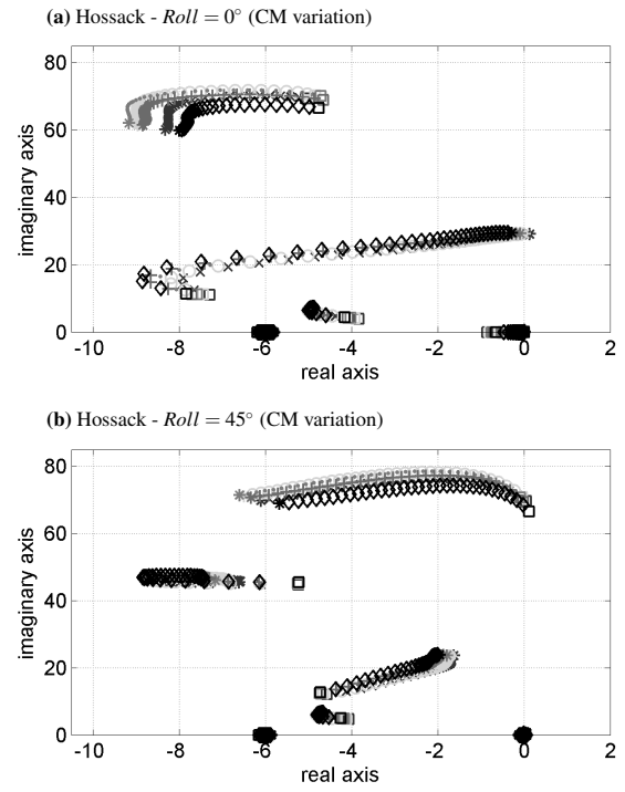
Fig. 31: Root loci for the Hossack suspension system in which its centre of mass is displaced towards the steering axis. 68mm forward (blue ×), 34mm forward (green ○), 0mm (magenta ·) -34mm backwards (red +) and -68mm backwards (black ◇)
