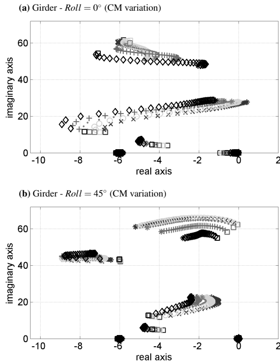
Fig. 30: Root loci for the Girder suspension system in which its centre of mass is displaced towards the steering axis. 68mm forward (blue ×), 34mm forward (green ○), 0mm (magenta ·) -34mm backwards (red +) and -68mm backwards (black ◇)
