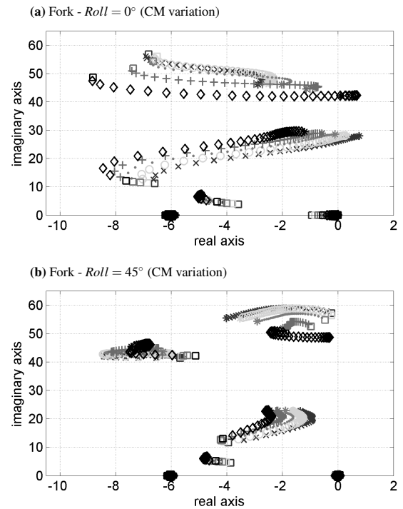
Fig. 32: Root loci for the telescopic fork suspension system in which its centre of mass is displaced towards the steering axis. 68mm forward (blue ×), 34mm forward (green ○), 0mm (magenta ·) -34mm backwards (red +) and -68mm backwards (black ◇)
