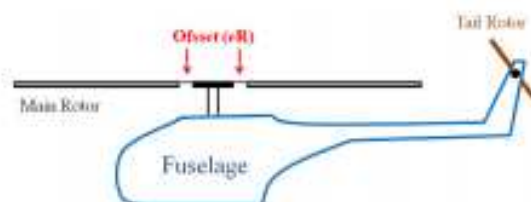
Fig. 1. Helicopter model with "offset" flap hinge indicated.
