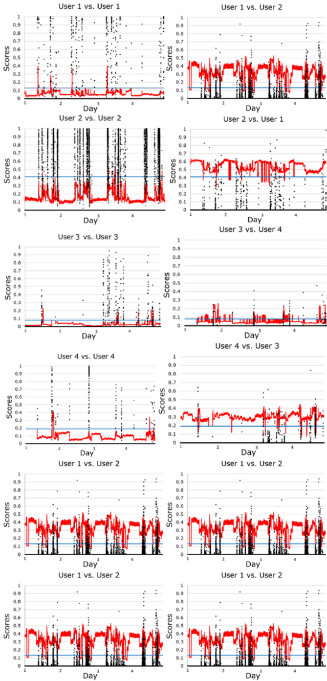
Figure 2: Graphs when a trained adaptive threshold scheme is tested on a genuine and impostor users. The graphs depict the scores of touchscreen gestures as black dots, the dynamic threshold as a red line, and the static threshold as a blue line.
