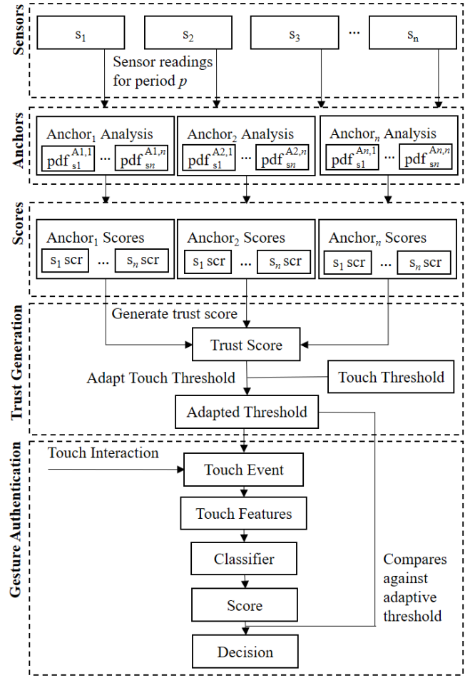
Figure 1: The framework for our proposed adaptive threshold scheme. The symbol pdf represents a probability density function which scores sensor s_n readings for an anchor An,n producing a score s_nsrc .
