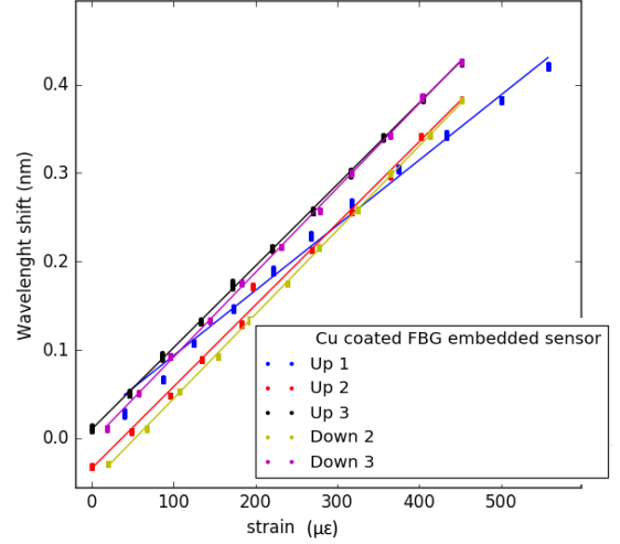
Fig. 12. Strain characterization for embedded Cu coated fiber optic sensors. The sensitivities of each linear fit are: Up1: 0.0007\text{ nm}/\mu\epsilon , Up2: 0.0009\text{ nm}/\mu\epsilon , Up3: 0.0009\text{ nm}/\mu\epsilon , Down2: 0.0010\text{ nm}/\mu\epsilon and Down3: 0.0010\text{ nm}/\mu\epsilon .
