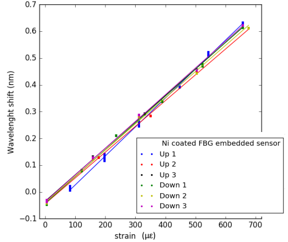
Fig. 13. Strain characterization for embedded Ni coated fiber optic sensors. The sensitivities of each linear fit are: Up1: 0.0011\text{ nm}/\mu\epsilon , Up2: 0.0010\text{ nm}/\mu\epsilon , Up3: 0.0010\text{ nm}/\mu\epsilon , Down1: 0.0010\text{ nm}/\mu\epsilon , Down2: 0.0010\text{ nm}/\mu\epsilon and Down3: 0.0010\text{ nm}/\mu\epsilon .
