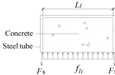
Figure 15 Equilibrium diagram of cross-sectional forces
