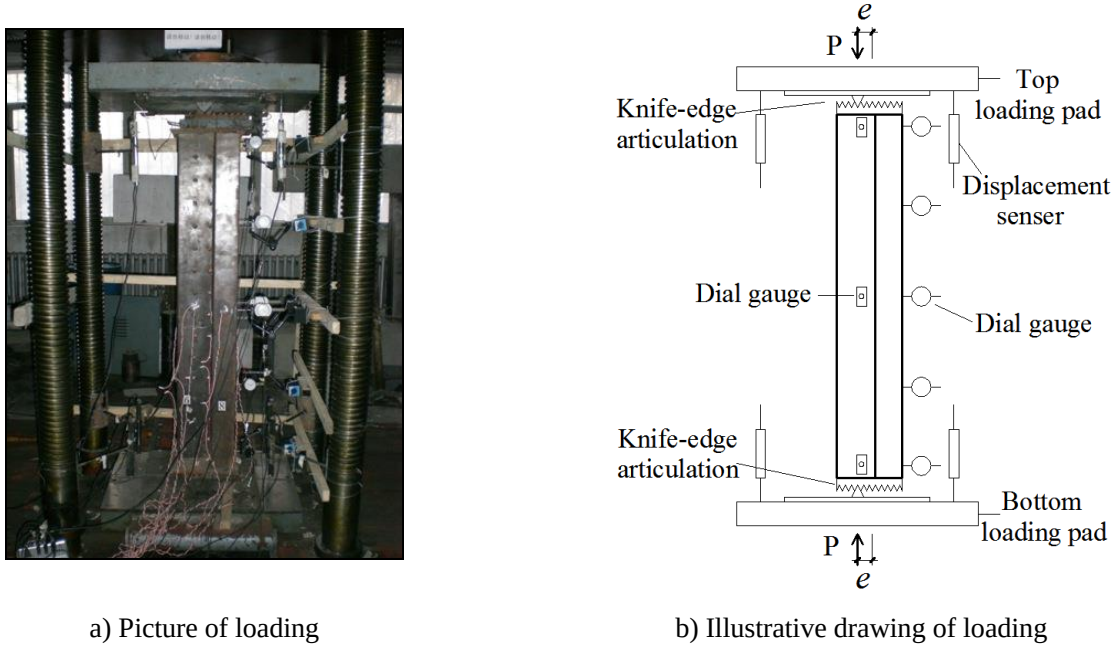
Figure 5. Loading devices and measuring apparatus in eccentric compressive test
