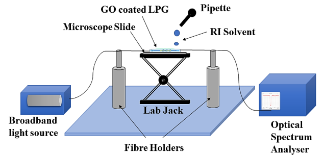
Fig. 6. Experimental setup used for external RI sensing measurements
