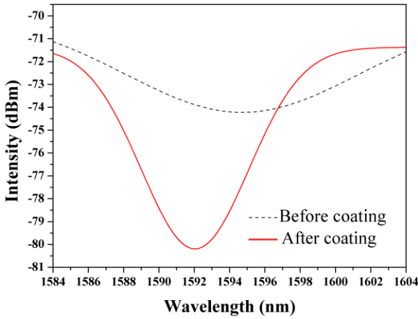
Fig. 4. Transmission spectra of the LPG before and after coating in the wavelength region 1584 nm to 1604 nm
