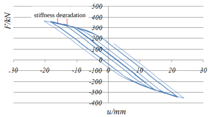
b Hysteric-curve from numerical model
