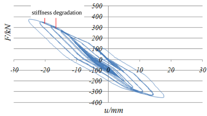
a Hysteric-curve from test
