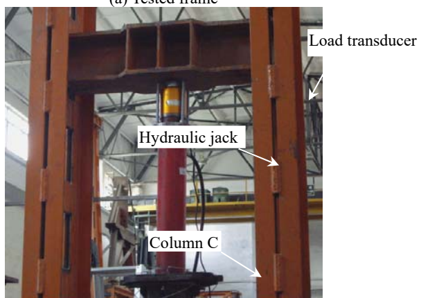
(b) Loading equipment
