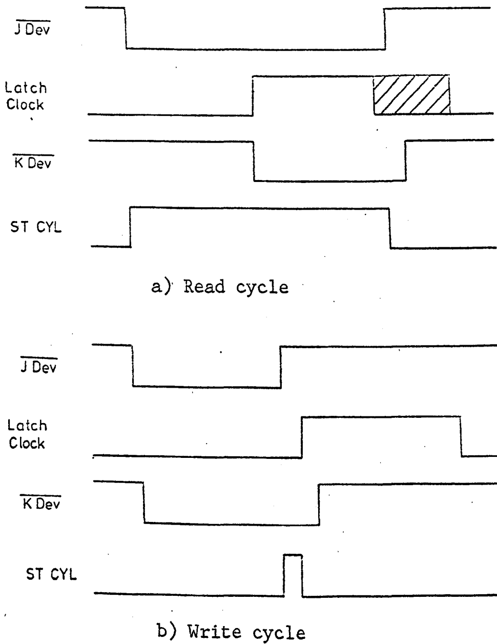
Figure 3.13 Read and write handshake sequences.
