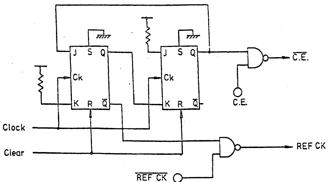
Figure 3.24 \overline{\text{C.E.}} and REF CK generator circuit for standby mode.
