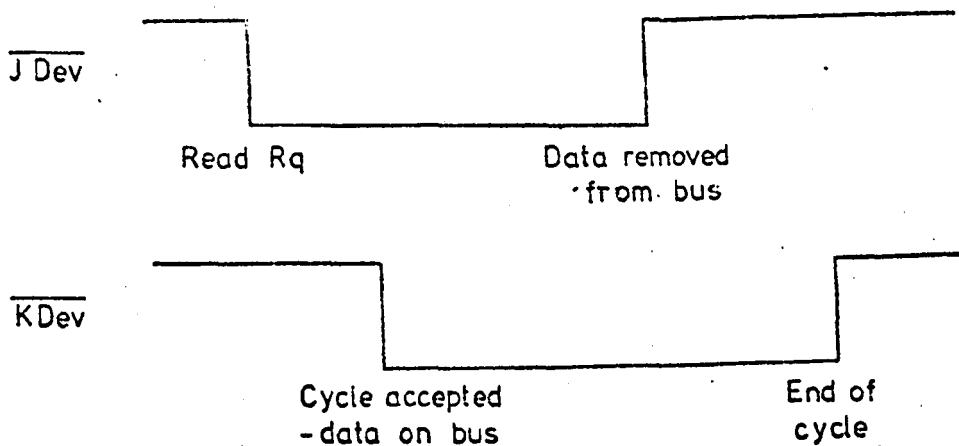
a) Read cycle
