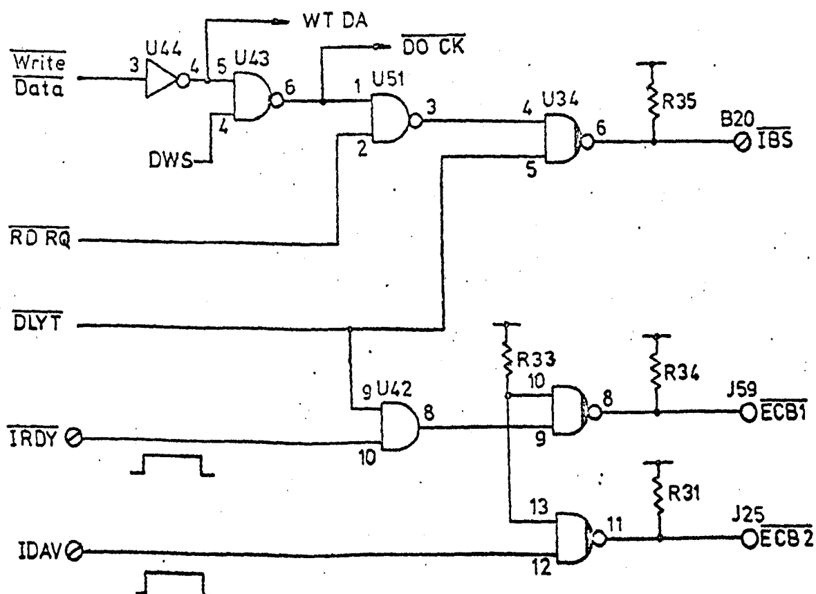
Figure 7.1.8 Handshake lines.
