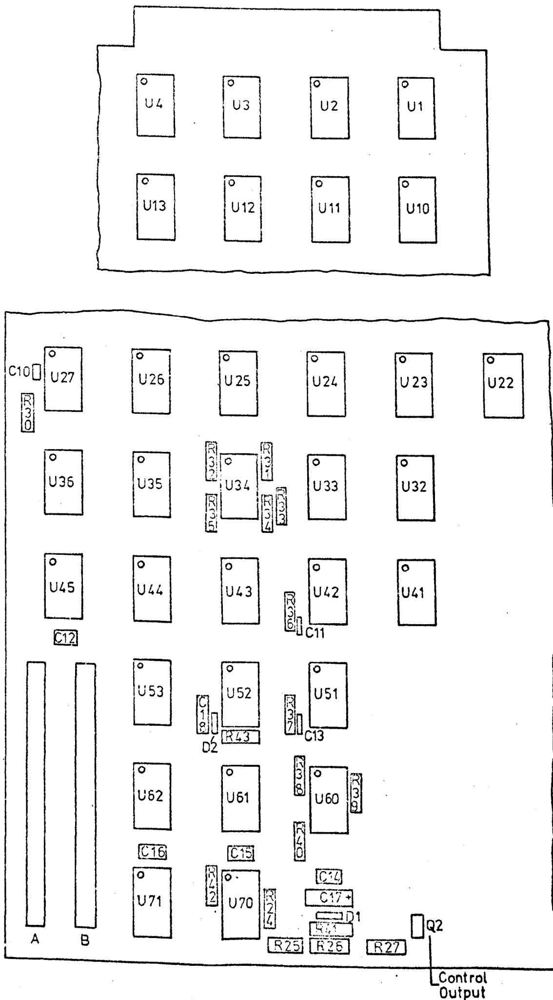
Figure 7.1.13 Cassette interface component layout.
