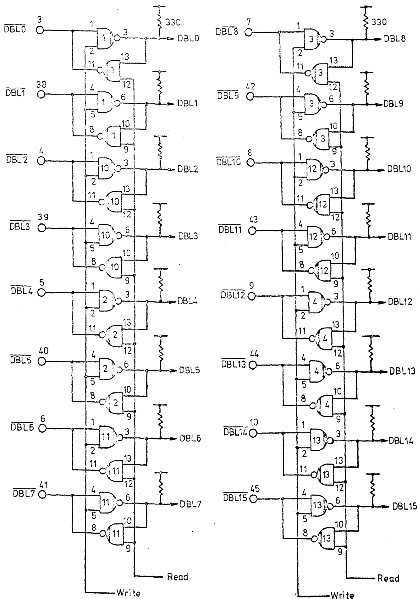
Figure 7.1.11 Bi-directional driver-receivers.
