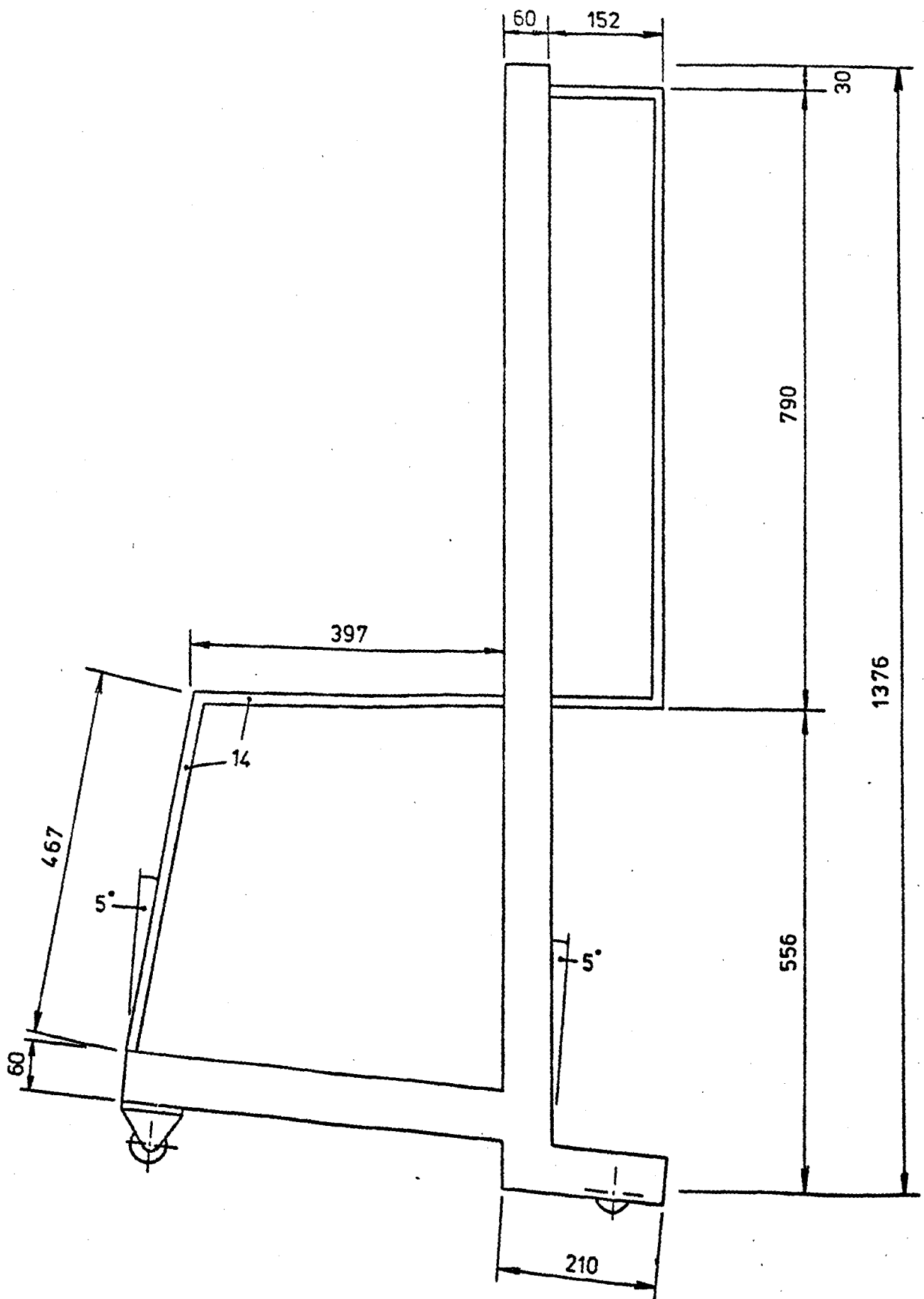
Figure 9.1 Mobile rack units - main dimensions.
