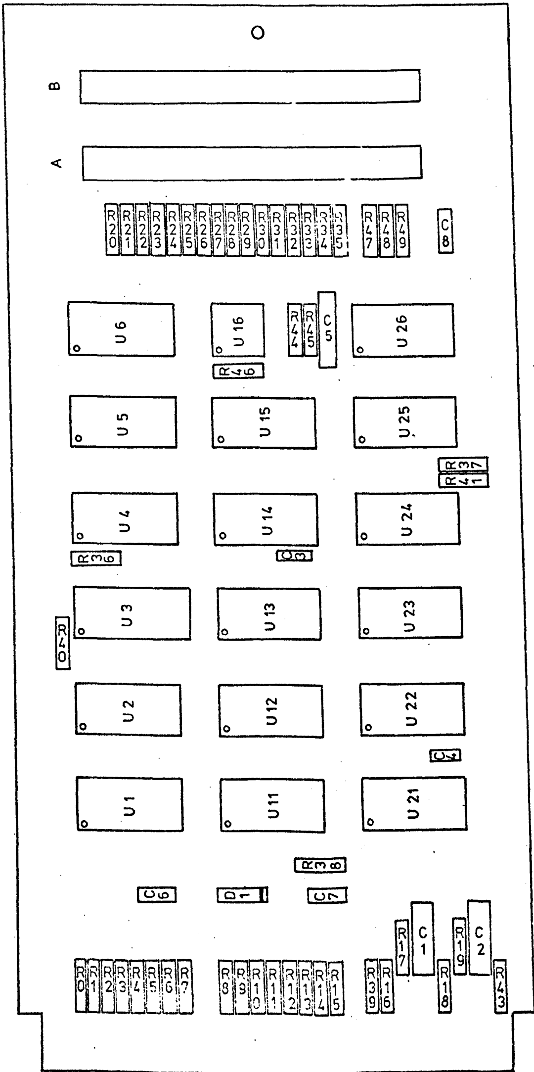
Figure 1.18 Component layout.
