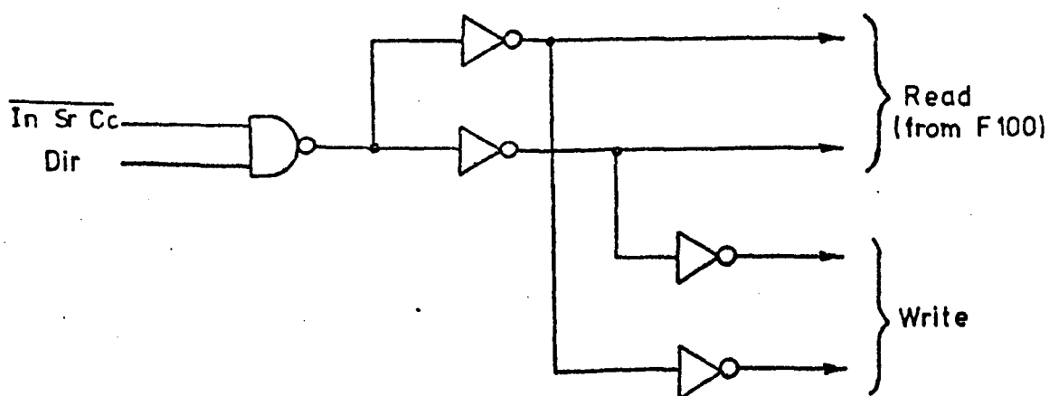
Figure 2.5 Read-write control.
