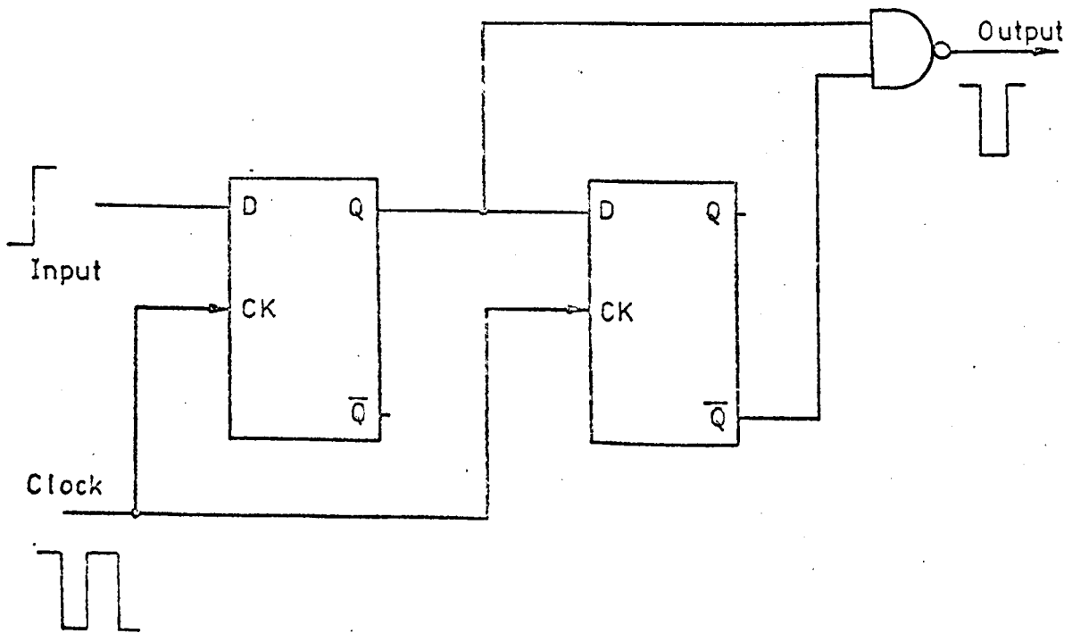
Figure 1.3 Edge-detector circuit.
