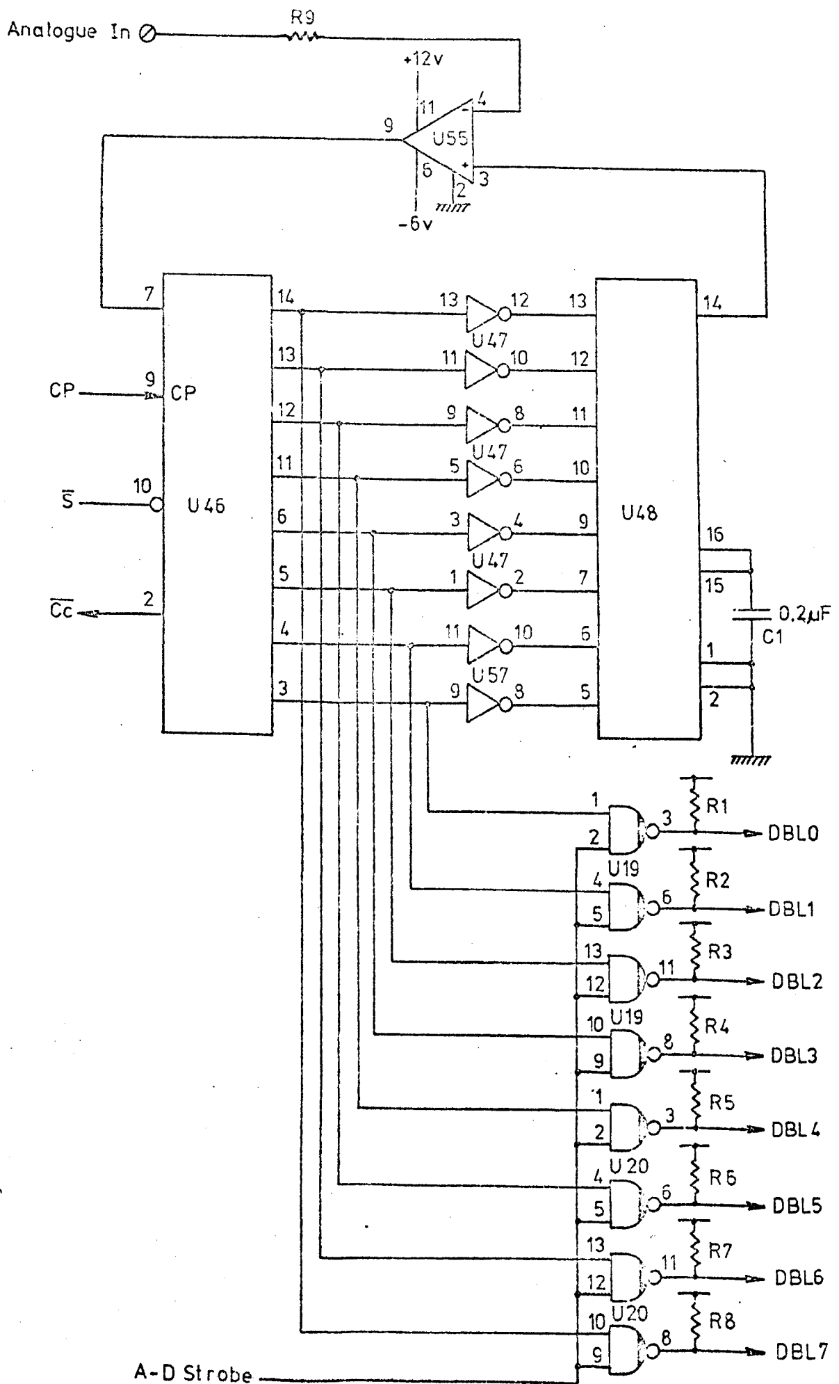
Figure 6.3 Successive approximation type A-D converter.
