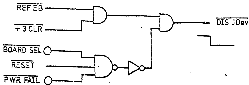
Figure 3.14. Disable inputs for \overline{\text{JDev}} signal.
