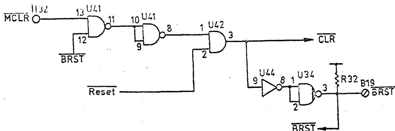
Figure 7.1.2 Reset circuit.
