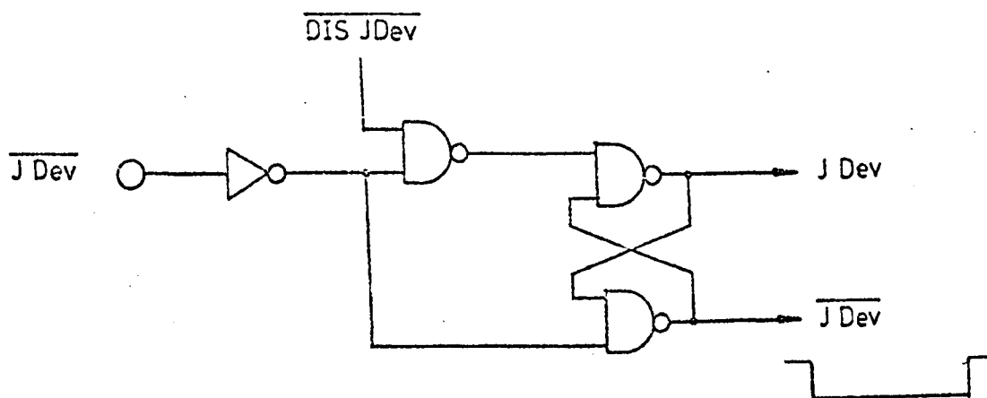
Figure 3.15 \overline{\text{JDev}} input circuit.
