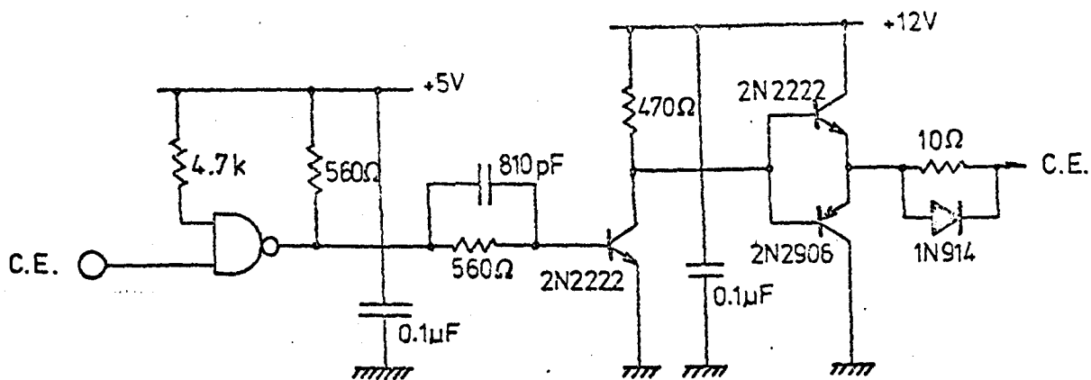
Figure 3.35 Chip enable driver circuit.
