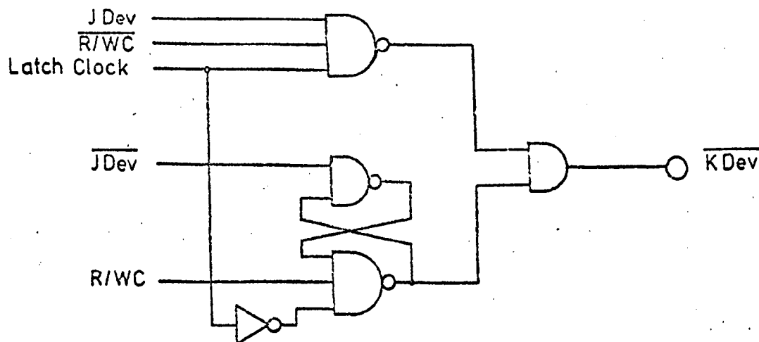
Figure 3.16 \overline{\text{KDev}} handshake circuit.
