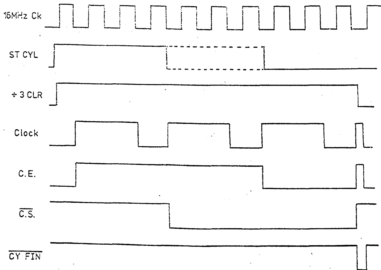
Figure 3.9 Complete clocking sequence for one cycle.
