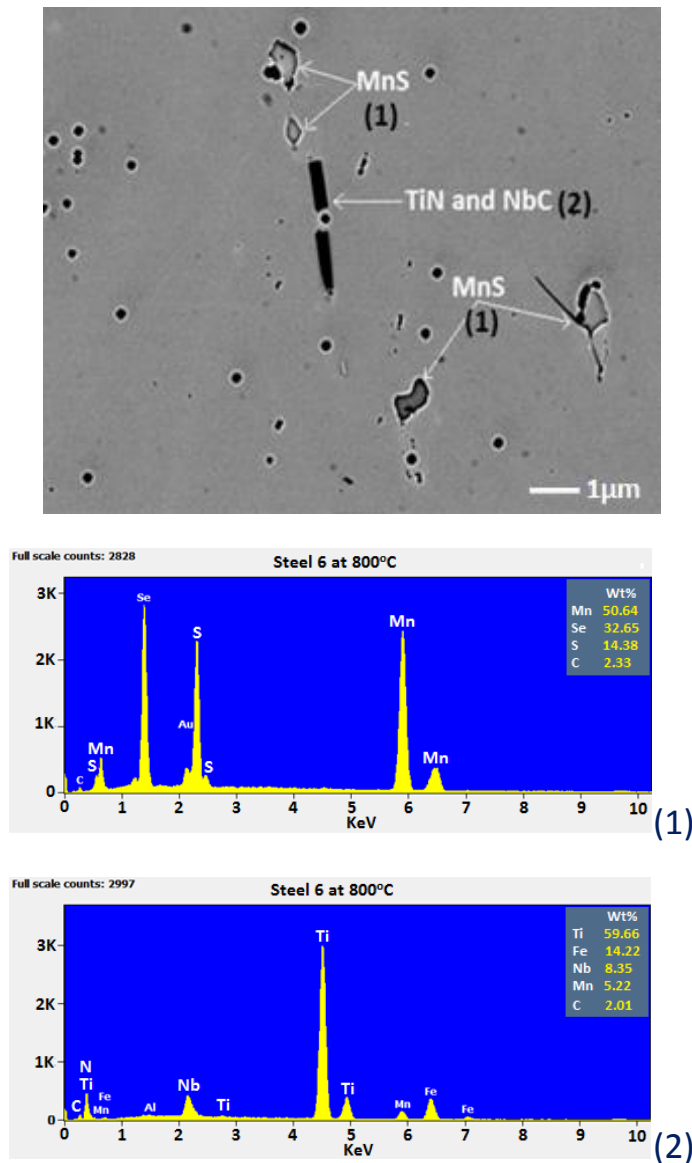
Fig. 8c. Higher Ti steel 6 tested at 800°C. Particles (1) are MnS. Particle (2) is a Ti-Nb nitride.
