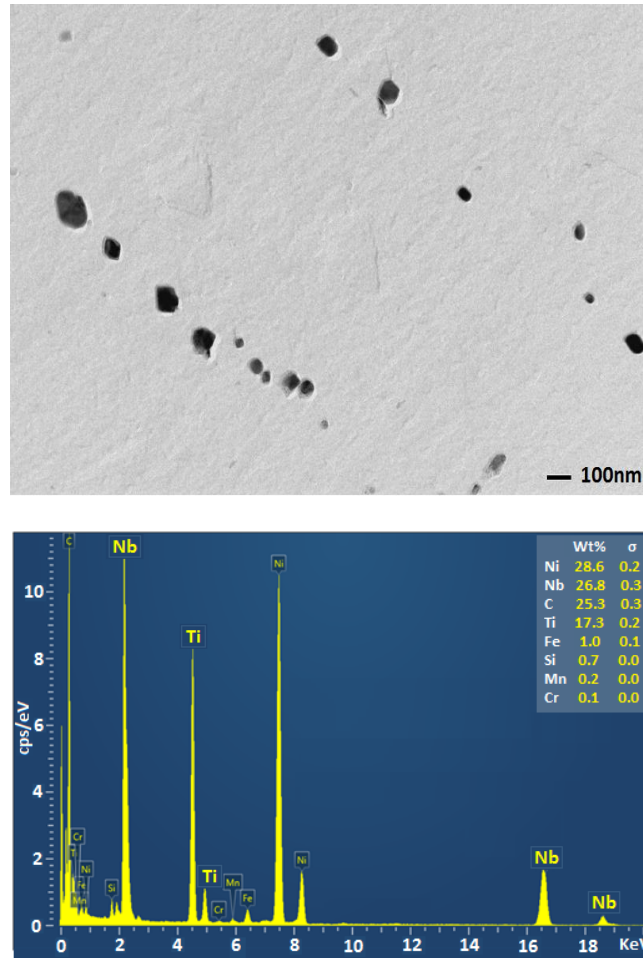
Fig 9a Nb-Ti carbonitrides found in steel 1 tested at 800°C. The precipitates varied considerably in size (~80nm in average size) but always gave similar composition.
