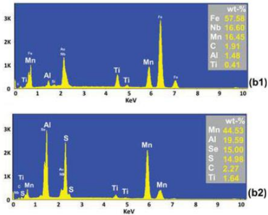
Fig. 8b. Steel 1, tested at 1000°C. Particles (1) AlN with Ti-Nb Nitrides and MnS. Particle (2), MnS with probably AlN and some TiN.
