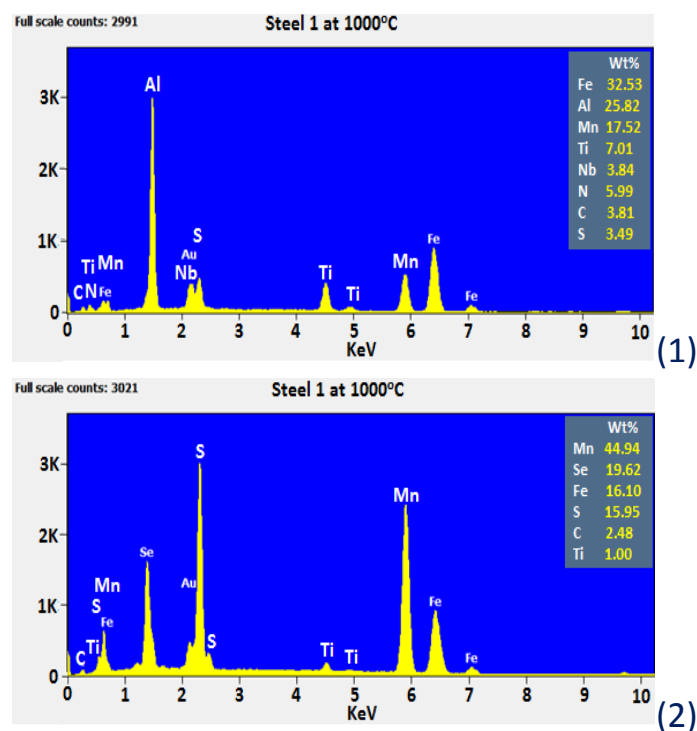
Fig.8a. Lower Ti steel 1, showing the likely presence of AlN on MnS inclusions. (AlN shows up as black in the photo and MnS as grey).The analysis spectrums show particle (1) AlN with Ti rich nitride. Particle (2) MnS with a Ti containing particle.
