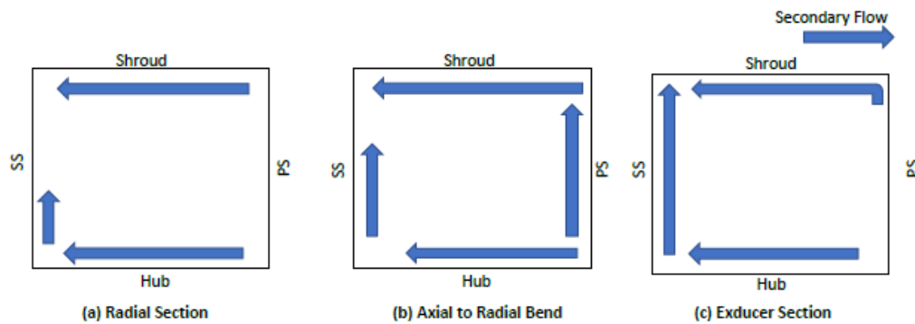
Figure 7: Secondary flow motion along turbine rotor passage
