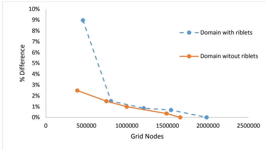
Figure 4: Grid independence study for computational domain with riblets
