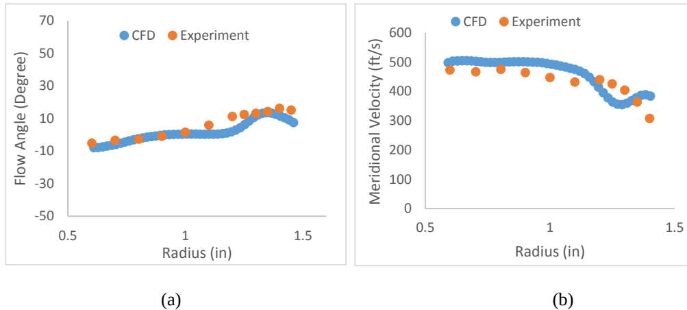
Figure 6: Spanwise distribution of (a) flow angle (b) meridional velocity at rotor discharge
