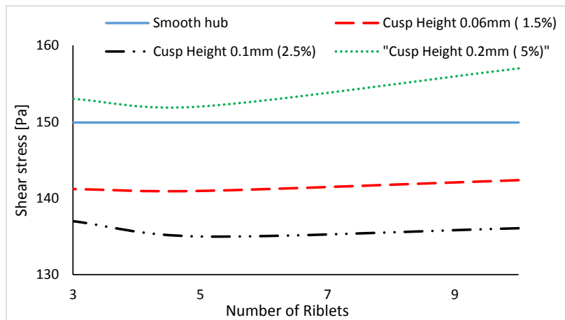
Figure 14: Wall shear stress comparison between different riblets geometries
