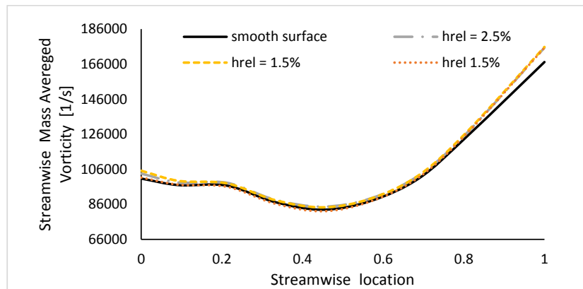
Figure 17: Mass averaged streamwise vorticity along rotor passage
