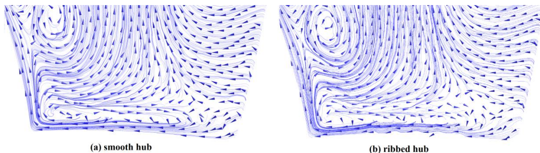
Figure 8: effect of riblets on cross stream motion of the low energy fluids near the hub surface
