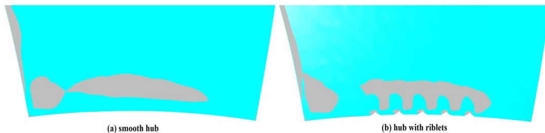
Figure 10: Stream-wise vortex structure over hub surface
