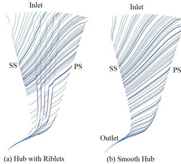
Figure 9: Limiting streamlines at the rotor hub
