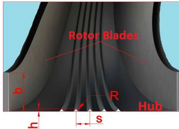
Figure 3: Riblets terminology
