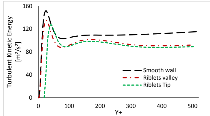
Figure 13: comparison of turbulent kinetic energy for both smooth rotor and rotor with riblets
