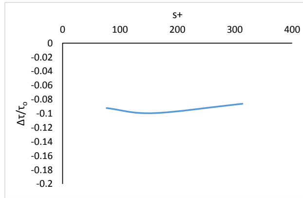
Figure 15: drag reduction for different riblets spacing
