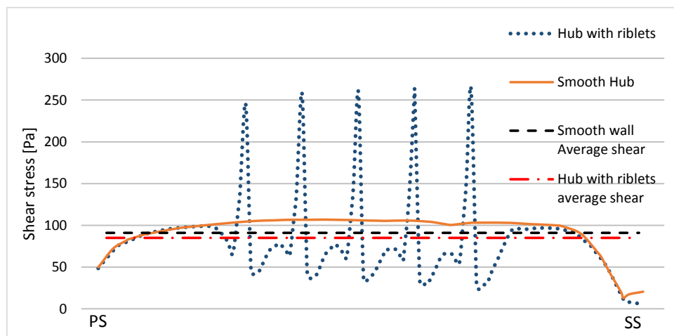
Figure 12: wall shear at the hub surface calculated at 40% stream-wise location
