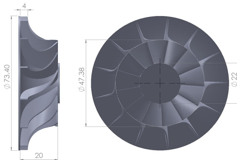
Figure 2: rotor dimensions [mm]
