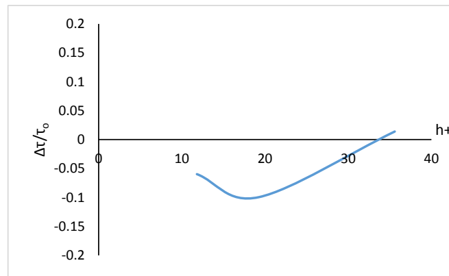
Figure 16: drag reduction for different riblets spacing
