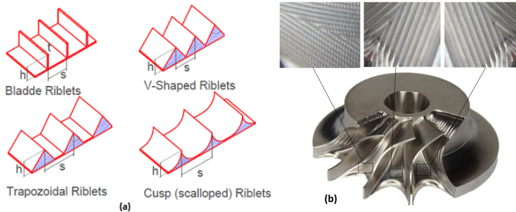
Figure 1: (a) Different riblet configurations (b) Turbine rotor with three different hub surface finish
