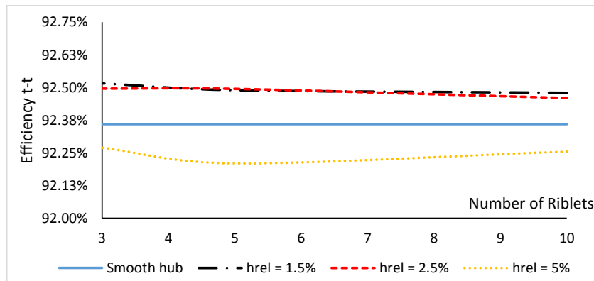
Figure 18: Turbine performance for different riblets geometry
