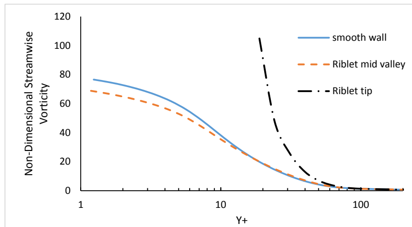
Figure 11: mass averaged streamwise vorticity at 40% stream-wise location
