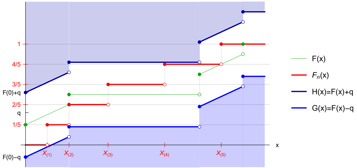
Figure 3: Illustration of the equivalence of P(F(x) - q \leq F_n(x) \leq F(x) + q, \text{ for all } x) to P\left(F^{-1}\left(\frac{i}{n} - q\right) \leq X_{(i)} \leq F^{-1}\left(\frac{i}{n} + q\right) \text{ for } 1 \leq i \leq n\right) (cf., Remark 4.2), for F(x) defined as in (23) with n = 5 .
