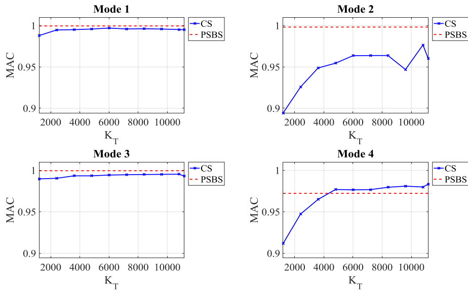
Figure 15: MAC versus reconstruction sparsity level K_T , obtained from the two considered approaches (i.e., PSBS-based and CS-based FDD) for CR= 31\%
