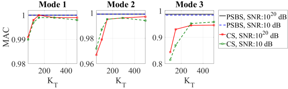
Figure 9: MAC versus reconstruction sparsity level K_T , obtained from the two considered approaches, PSBS-based and CS-based FDD, for CR= 31% and SNR= \{10^{20}, 10\} dB
