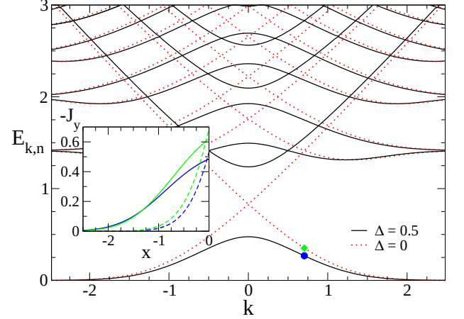
Figure 3. Edge states for a semi-infinite ( x < 0 ) graphene sheet with V = 0 and armchair conditions at x = 0 . Main panel: Dispersion relation for \Delta = 0.5 E_B (solid black) and for \Delta = 0 (red dotted curves). Inset: Current density J_y(x) [in units of -ev_F ] vs position x/l_B for the two degenerate eigenstates (solid and dashed curves for s = + and s = - , resp.) with kl_B = 0.705 . Blue (green) curves are for \Delta/E_B = 0.5 ( \Delta = 0 ) with E_{k,n,s}/E_B \simeq 0.2683 ( \simeq 0.3520 ), cf. the blue circle (green diamond) in the main panel.
