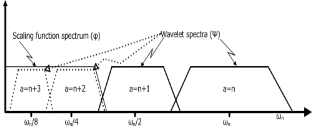
Fig. 6.3: Use of scaling function \varphi to cover the low frequency part of the signal
