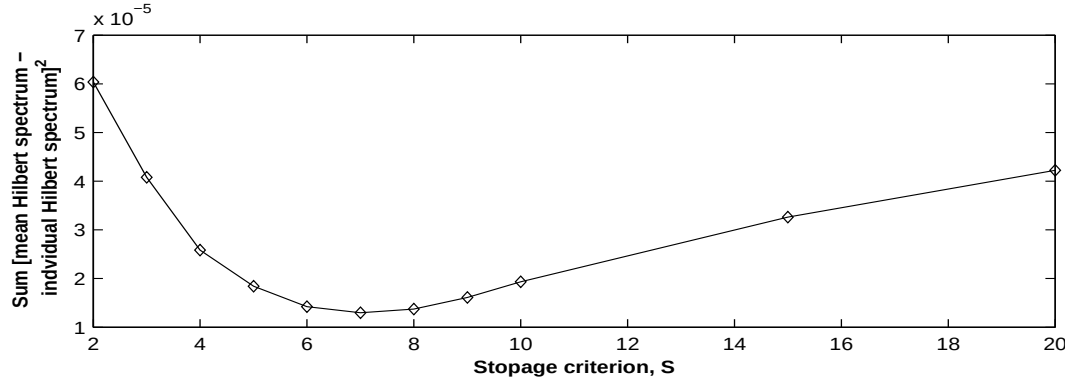
Fig. 14.3: Squared deviation obtained using the mean Hilbert spectrum and the individual Hilbert spectrum for the stoppage criterion S values of 2-10, 15 and 20 in the case of simulated signal one
