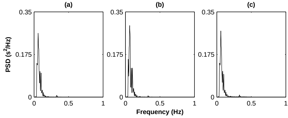
Fig. 8.25: Spectrum of the real HRV signal obtained using Welch's method (moving beat case); (a) spectrum of the original signal; (b) spectrum after moving five random beats from the signal; (c) spectrum after beat correction
