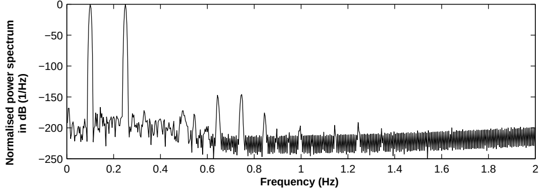
Fig. 8.11: Normalised Power Spectrum (NPS) obtained for the modulating signal of Eq. 8.13 with 5 minutes of data using Welch's periodogram method
