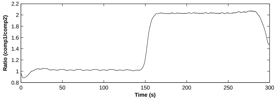
Fig. 12.7: Amplitude ratio between the two components of the second simulated signal. The change in the ratio value occurring almost at the middle of the data is in accordance with the simulation, where the amplitude of the HF component was halved mid way through the simulation
