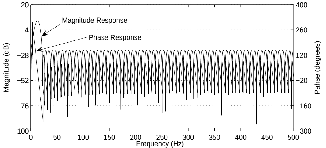
Fig. 5.2: Magnitude and Phase response of the bandpass filter used for QRS enhancement
