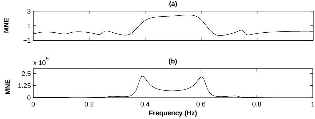
Fig. 8.18: MNE (a) after performing beat correction; (b) before beat correction. Signals are corrupted by removing five random beats
