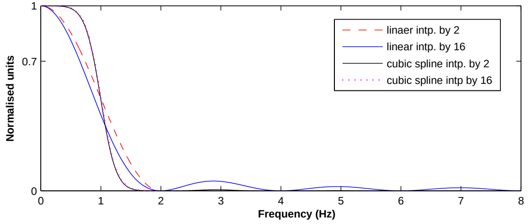
Fig. 8.2: Frequency response, linear interpolation (interp.) and cubic spline of order two and sixteen ( T_0=0.5 )
