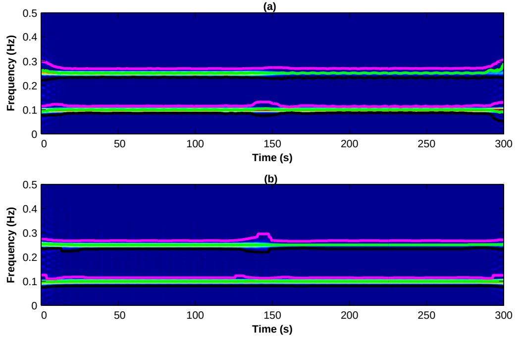
Fig. 13.6: Time-Frequency Representation (TFR) of the second simulated signal using (a) SPWVD ;(b) CWD. In each case the thick green lines represent the ICF for the two components present in the signal. Similarly the thick black and magenta lines represent the lower and the upper boundaries for the two components respectively
