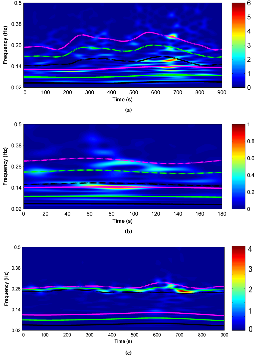
Fig. 12.19: Scalogram representation of the data obtained from a locally anaesthetised patient; (a) the representation for the data segment fifteen minutes before the application of the anaesthetic block, (b) the representation for the data obtained during the application of the block, (c) the representation of the data obtained fifteen minutes after the application of the block. In each case the ICF and the boundaries related to the HF band are represented by dashed line while boundaries and ICF related to the LF band are represented by solid lines
