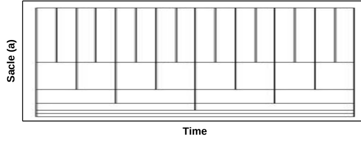
Fig. 9.10: Wavelet packet tiling in time-frequency plane
