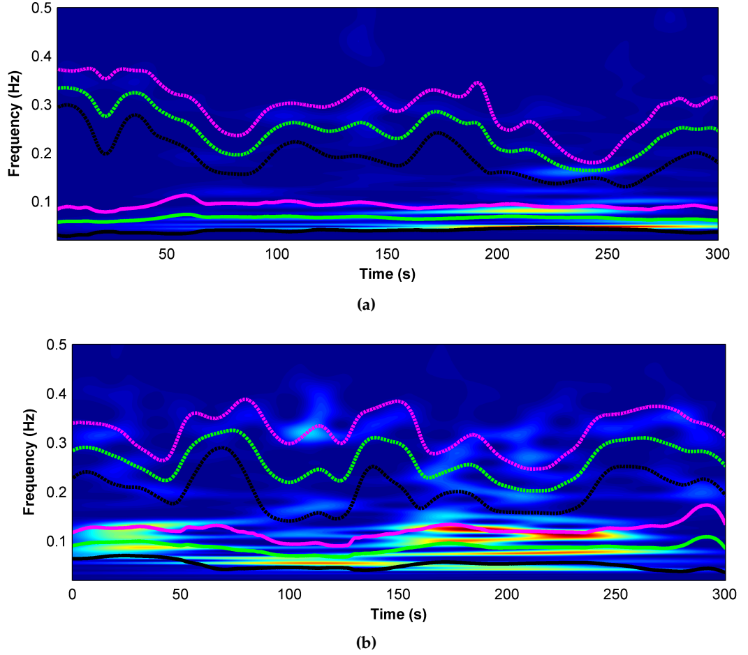
Fig. 12.15: Scalogram of the two HRV signals associated with the data segment used to generate the results of Fig. 12.14. In both cases the ICF and the boundaries related to the LF and HF band are also shown. The dashed lines represent the HF band boundaries and the ICF related to respiration and the solid lines represent the same information for the LF region of the HRV signal
