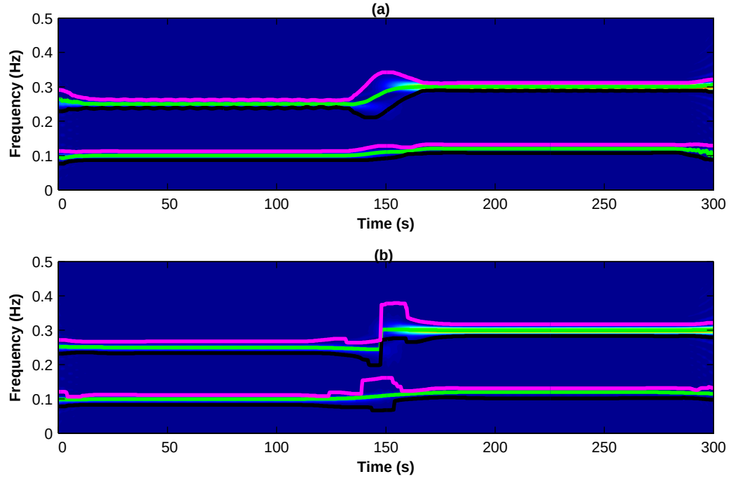
Fig. 13.10: Time-Frequency Representation (TFR) of the fourth simulated signal using (a) SPWVD ;(b) CWD. In each case the thick green lines represent the ICF for the two components present in the signal. Similarly the thick black and magenta lines represent the lower and the upper boundaries for the two components respectively
