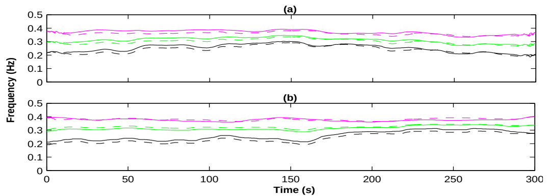
Fig. 13.14: ICF and the respiration boundaries calculated using actual respiration signal (solid lines) and respiration signal estimated from the ECG signal (dashed lines) from two elderly volunteers from "Fantasia Database". The ICF was calculated using Eq. 11.2 and the boundaries for the respiration component was defined as ICF \pm SDSE (see Eq. 11.3)
