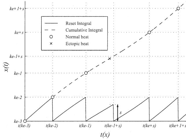
Fig. 8.7: Beat occurrence time generation in presence ectopic beat from the integral of the IPFM model [116]
