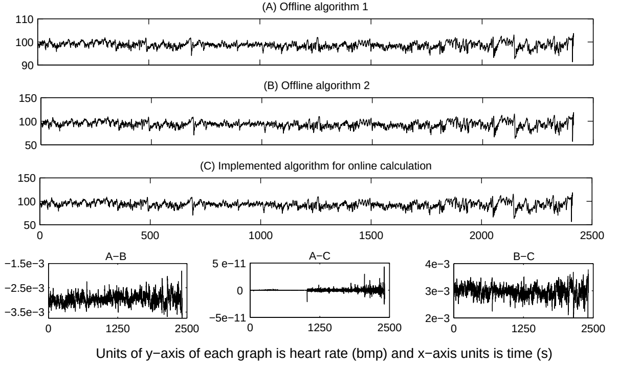
Fig. 8.5: Comparison results between two offline implementations of Berger et. al. algorithm with the version implemented for online calculation
