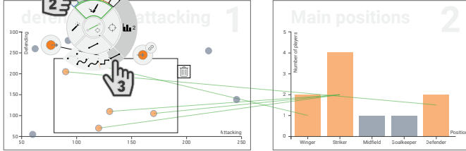
(E) CONFIGURE TARGET (1) De-aggregating the target and (2) setting its outline color to brown shows the individual target data points within the aggregated bars. The chain link symbol indicates that the coupling with the source is broken.
