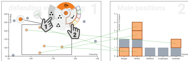
Fig. 2. The basic functionality of MyBrush illustrated using a scatterplot of attacking vs. defending skills in which each circle represents a soccer player (View 1, left) and a barchart of player positions on the soccer field (View 2, right). We demonstrate support for personal agency in the creation and configuration of a single brush in View 1.
