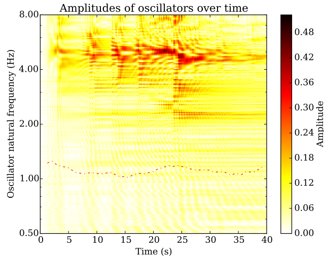
(A) GFNN response to unfiltered, log-scaled CSD.
