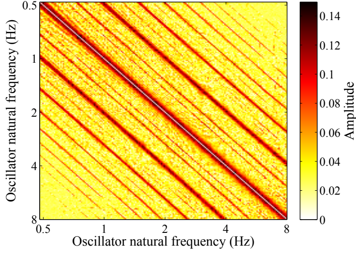
FIGURE 2.5: Amplitudes of a GFNN connection matrix, showing connections formed at high-order integer ratios.
