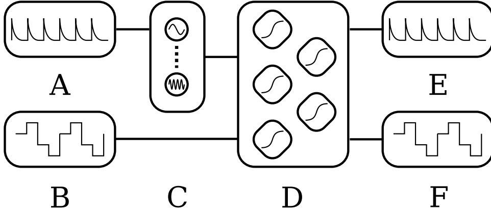
FIGURE 3.7: Network diagram for LSTM3b and LSTM3c showing (A) note onset sequence, (B) scale degree sequence, (C) GFNN, (D) LSTM, (E) note onset prediction, and (F) scale degree prediction.
