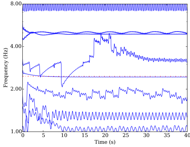
FIGURE 6.2: AFNN frequencies adapting to a sinusoidal stimulus. The dashed line shows stimulus frequency.
