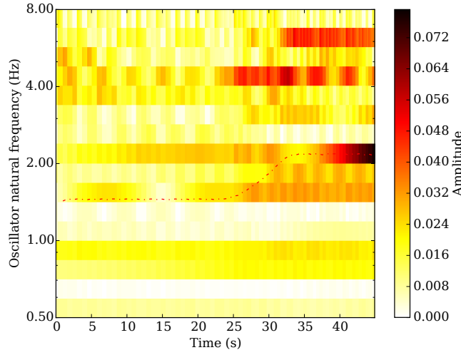
FIGURE 6.1: LD-GFNN (4opo) output. The dashed line shows stimulus frequency.
