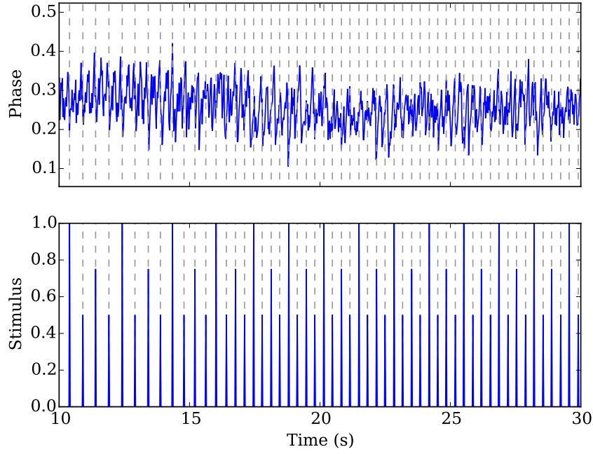
FIGURE 6.3: WPO of the AFNN over time. Reduced interference can be seen compared with Figure 5.2.
