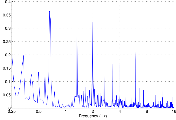
FIGURE 2.4: An example magnitude spectrum of a summed GFNN output.
