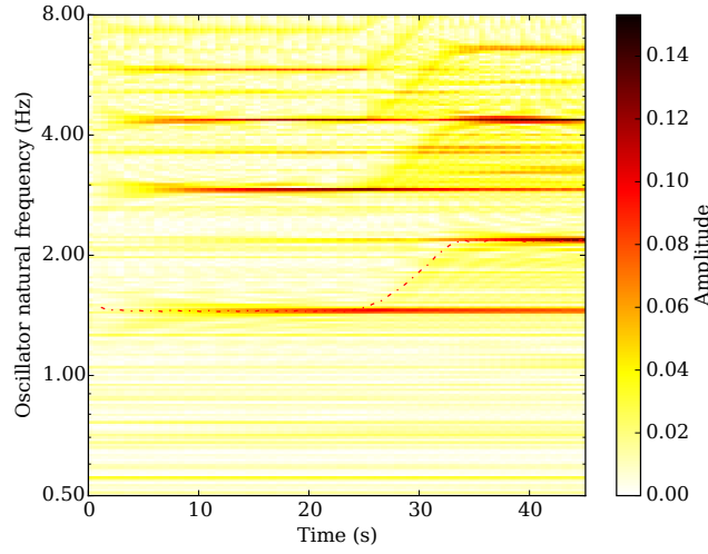
FIGURE 5.1: Amplitudes of oscillators over time. The dashed line shows stimulus frequency. The stimulus itself is shown in Figure 5.2. There is an accelerando after approximately 25s.
