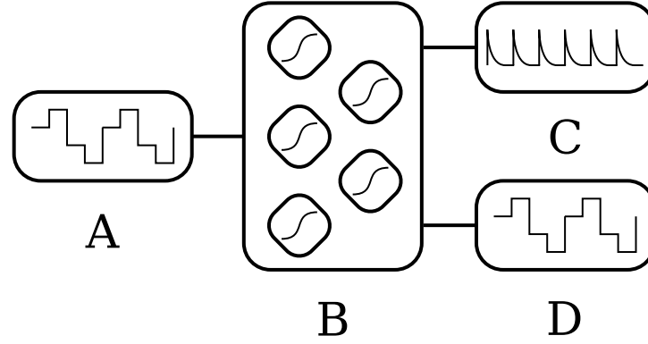
FIGURE 3.6: Network diagram for LSTM3a showing (A) scale degree sequence, (B) LSTM, (C) note onset prediction, and (D) scale degree prediction.
