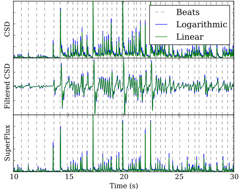
(A) A comparison of mid-level representations of an excerpt of Mazurka 06-1, performance ID 9048-01.
