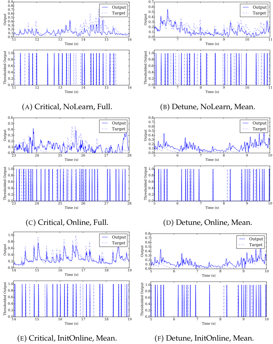
FIGURE 4.6: Example outputs from various trained networks over time.
