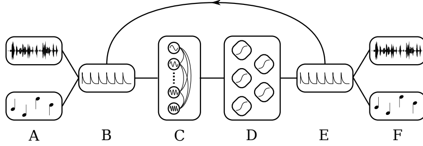
FIGURE 8.1: An overview of the proposed model showing (A) audio or symbolic input, (B) time-series rhythm representation, (C) AFNN, (D) LSTM, (E) time-series rhythm prediction, and (F) audio or symbolic output. An internal feedback loop connects E and B.
