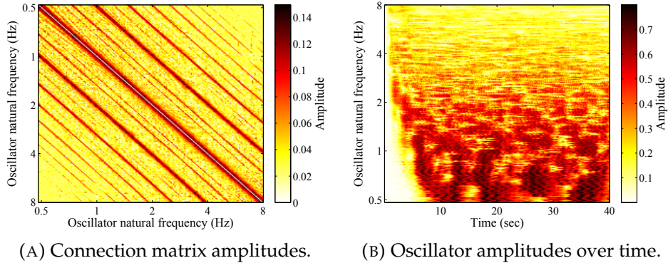
FIGURE 4.4: GFNN connection matrix learned in limit cycle mode and oscillator amplitudes with fixed connections.
