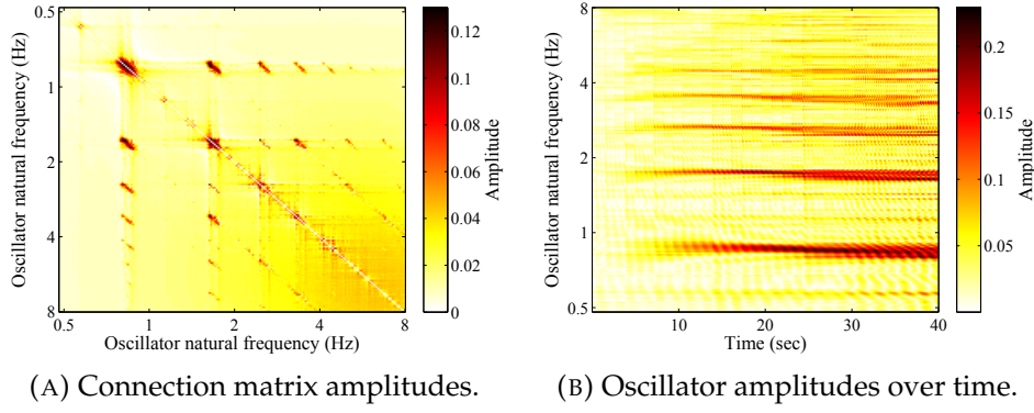
FIGURE 4.3: GFNN connection matrix and oscillator amplitudes with online learning.
