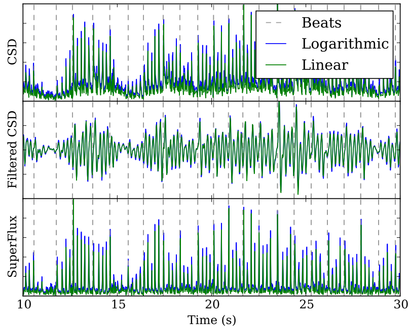
(B) A comparison of mid-level representations of an excerpt of SMC_003.
