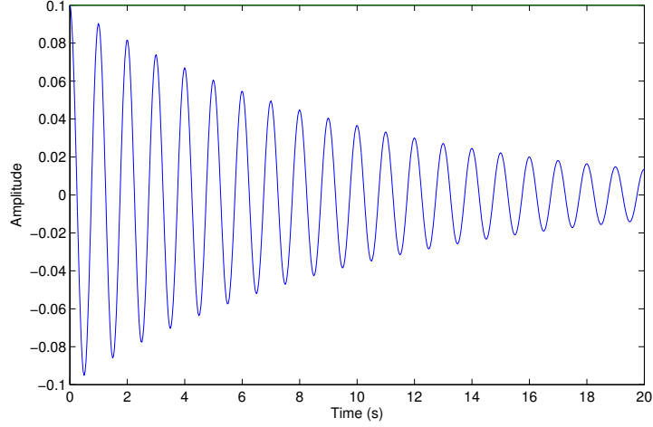
FIGURE 2.3: A canonical oscillator without stimulus, and with the following parameters, \omega = 2\pi, \alpha = -0.1, \beta_1 = 0, \beta_2 = -0.1, \delta_1 = 0, \delta_2 = 0, \varepsilon = 0.5, c = 0, x(t) = 0
