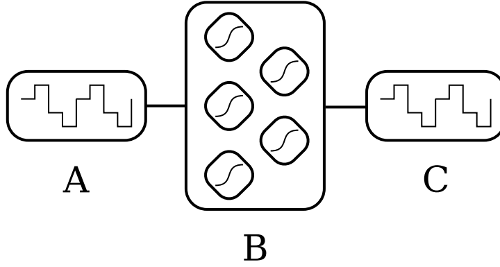
FIGURE 3.3: Network diagram for LSTM1a showing (A) scale degree sequence, (B) LSTM, and (C) scale degree prediction.
