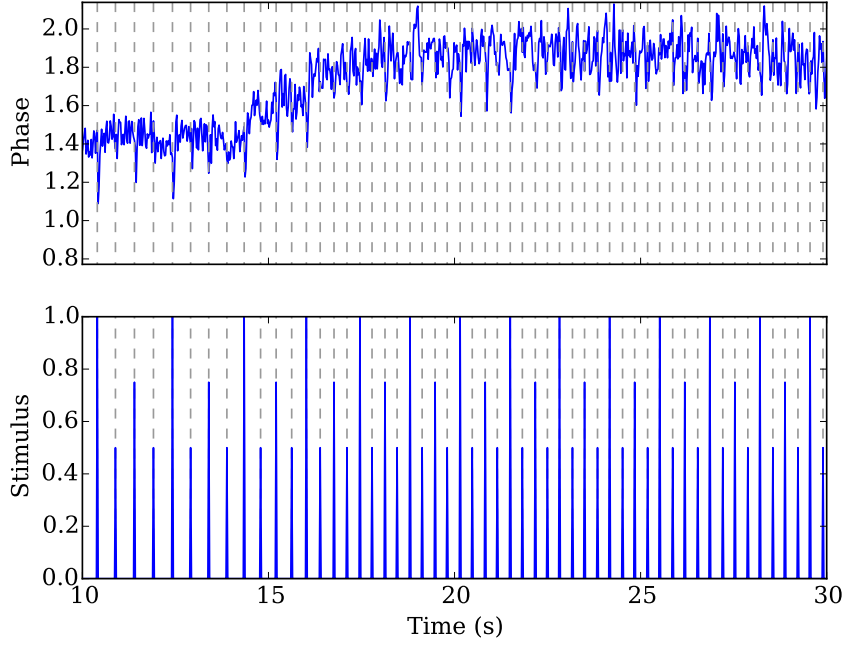
FIGURE 5.2: WPO of the GFNN over time. The stimulus is the same as Figure 5.1.
