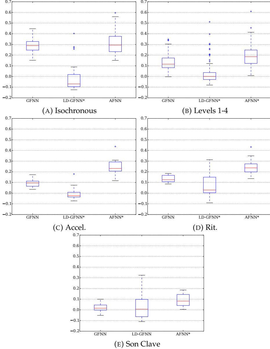
FIGURE 6.4: Box and Whisker plots of the PCC results. Boxes are as in Figure 5.4. *Denotes significance in a Wilcoxon signed rank test ( p < 0.05 ), compared with (A).
