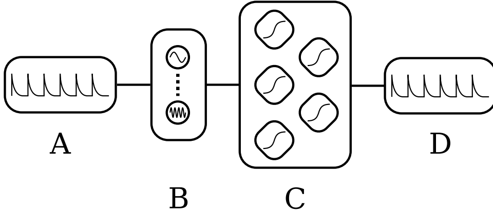
FIGURE 3.5: Network diagram for LSTM2a and LSTM2b showing (A) note onset sequence, (B) GFNN, (C) LSTM, and (D) note onset prediction.
