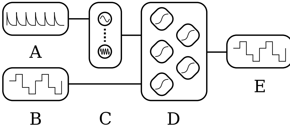
FIGURE 3.4: Network diagram for LSTM1b and LSTM1c showing (A) note onset sequence, (B) scale degree sequence, (C) GFNN, (D) LSTM, and (E) scale degree prediction.
