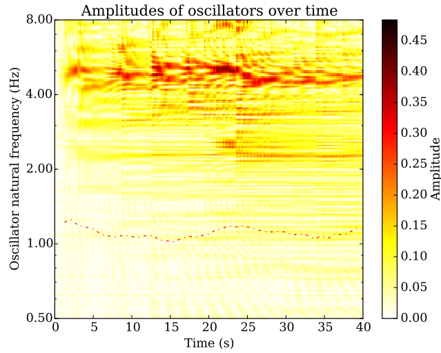
(C) GFNN response to unfiltered, log-scaled SuperFlux.
