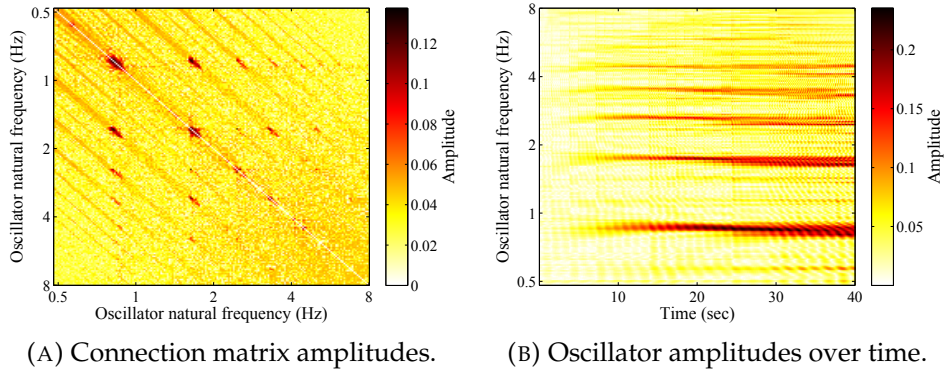
FIGURE 4.5: GFNN connection matrix and oscillator amplitudes with online learning and an initial state from Figure 4.4a.
