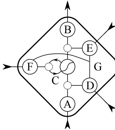
FIGURE 2.7: A single LSTM memory block showing (A) input, (B) output, (C) CEC, (D) input gate, (E) output gate, (F) forget gate and (G) peephole connections.
