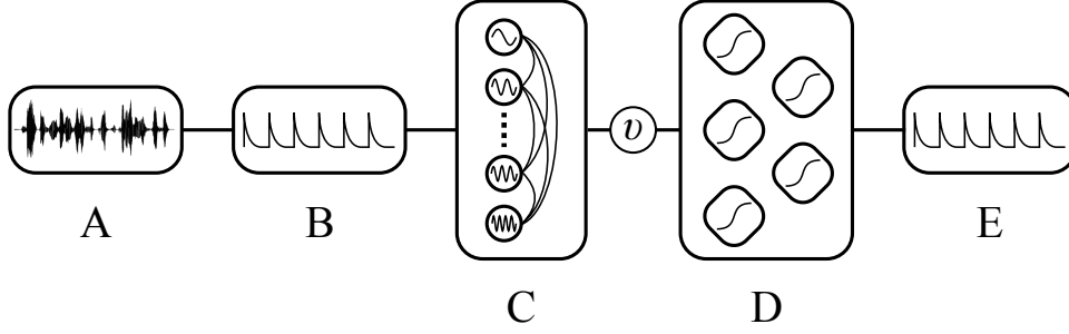
FIGURE 4.1: An overview of the GFNN-LSTM system showing (A) audio input, (B) mid-level representation, (C) GFNN, (D) LSTM, and (E) rhythm prediction output. The variable \nu can be a mean field function or full connectivity.
