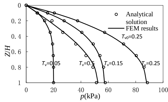
Fig.3 Comparison of pore pressure
