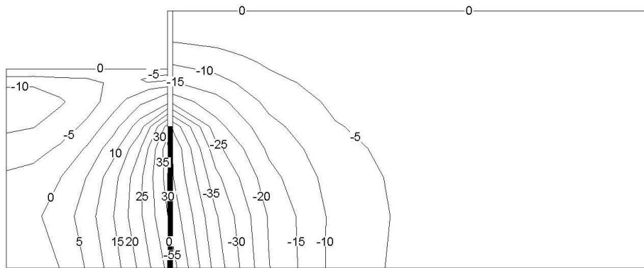
Fig.18 Distribution of excess pore-water pressures under BE (unit: kPa)
