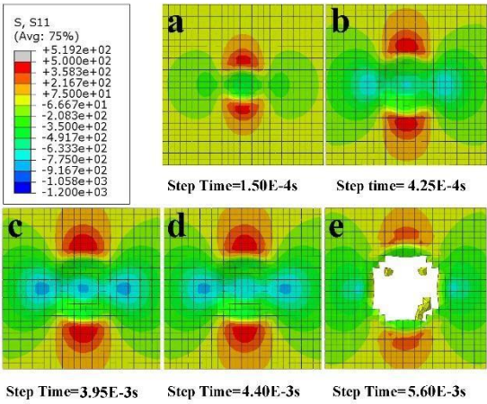
Fracture behaviour during long-duration peening
