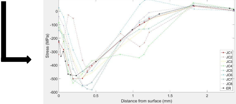
Influence of JC model parameters on peening residual stress
