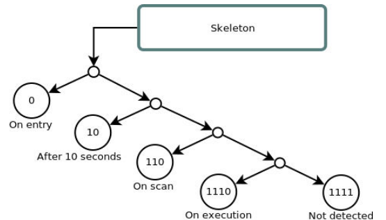
FIG. 2. THE POSSIBLE RESULTS OBTAINED ON A VM(a,o) . 0 MEANS DETECTION (NO FAILURE); 1 MEANS NO DETECTION (FAILURE).
