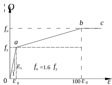
(a) Steel
