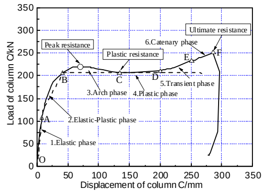
(b) Vertical load-displacement of middle column relationship curve Fig. 23 Test of semi-rigid composite frame under column loss [17]
