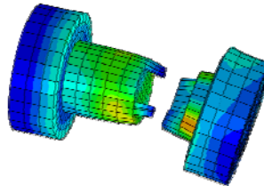
(e) Bolt fractured
