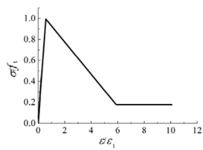
(c) Concrete in tension
