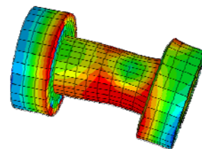
(c) Strength degradation progressed
