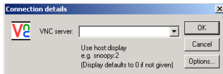
Figure 4.5 VNC viewer
