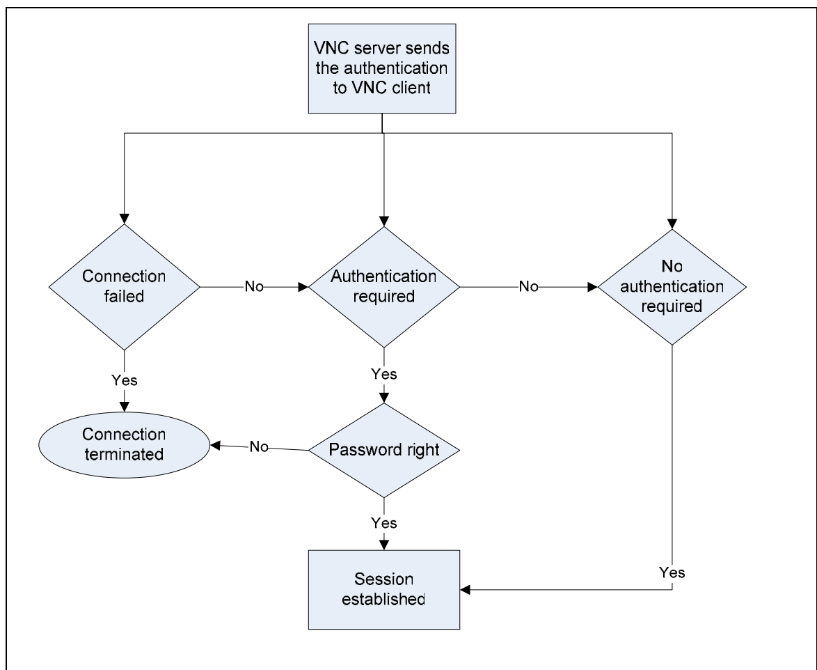
Figure 3.7 Authentication scheme
