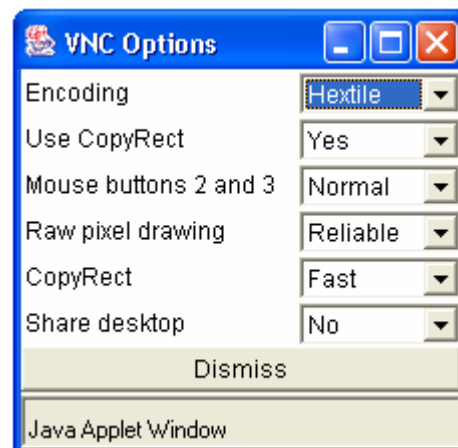
Figure 4.10 VNC options
