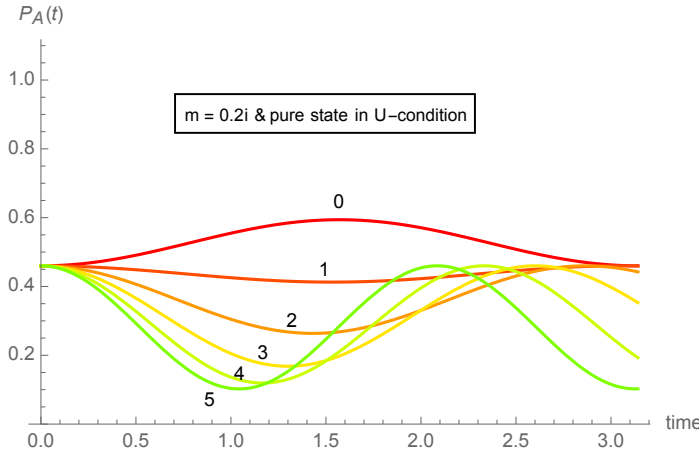
Figure 8. Outcome probability to continue based on Hamiltonian dynamics with Pauli matrix combination \vec{w} = \{.9, 0, 1\} in w -space and \vec{l} = \{-.5, 0, 1\} in l -space, and with an initial pure state in u -condition specified by p_w = .6 , p_{cw} = .7 and p_{cl} = .1 . The mixing parameter is varied, m = 0 to 1 in steps of 0.2 ( i=0 to 5 ).
