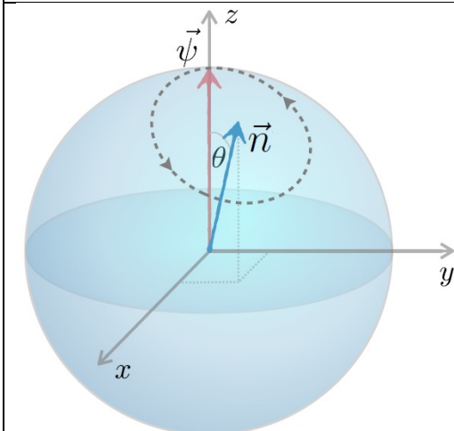
Figure 2e. Hamiltonian of the form H = n_x \sigma_x + n_y \sigma_y + n_z \sigma_z ; rotation axis \vec{n} at angle \theta to z-axis (i.e. it obtains from that in Figure 2c
