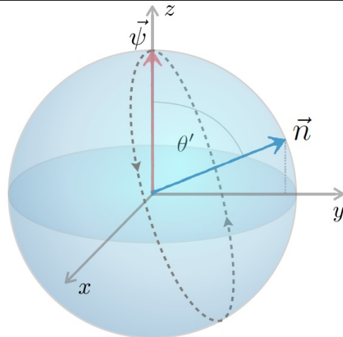
Figure 2d. Hamiltonian of the form H = n_y \sigma_y + n_z \sigma_z ; rotation axis \vec{n} in yz plane at angle \theta' to z-axis.
