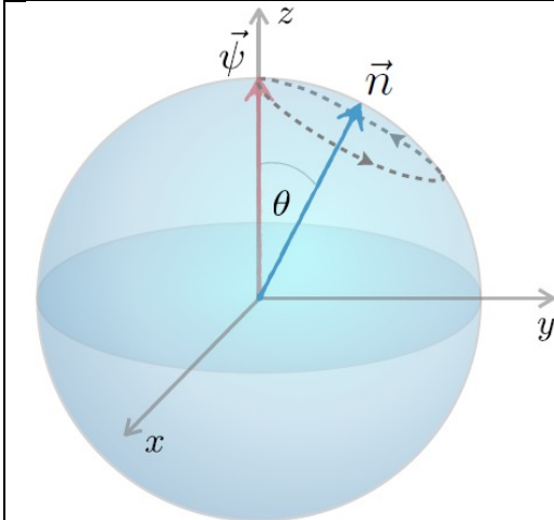
Figure 2c. Hamiltonian of the form H = n_y \sigma_y + n_z \sigma_z ; rotation axis \vec{n} in yz plane at angle \theta to z-axis.
