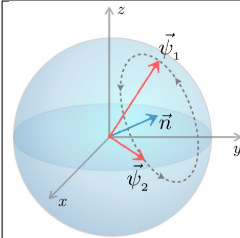
Figure 2a. For Hamiltonian H = \vec{n} \cdot \vec{\sigma} the state of the system traces a circle whose center is \vec{n} . Probability Prob_A(t) exhibits oscillatory behavior.
