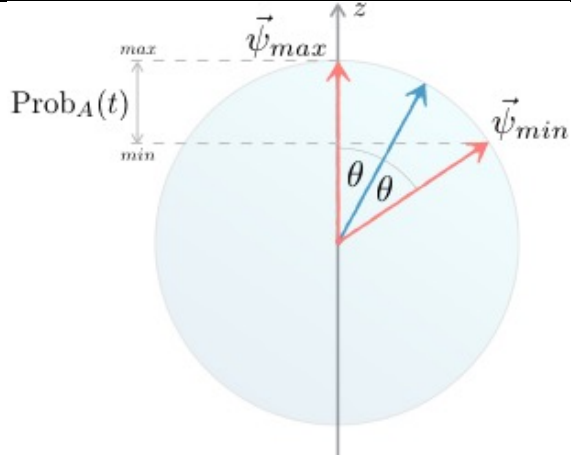
Figure 2g. Probability Prob_A(t) in Figures 2c and 2e oscillates between the maximum value equal to 1 and minimal value equal to \frac{1}{2}(1 + \cos 2\theta) = \cos^2 \theta .
