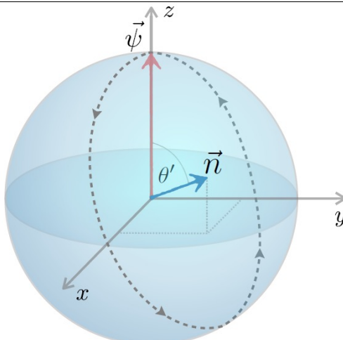
Figure 2f. Hamiltonian of the form H = n_x \sigma_x + n_y \sigma_y + n_z \sigma_z ; rotation axis \vec{n} at angle \theta' to z-axis (i.e. it obtains from that in Figure 2d by rotation
