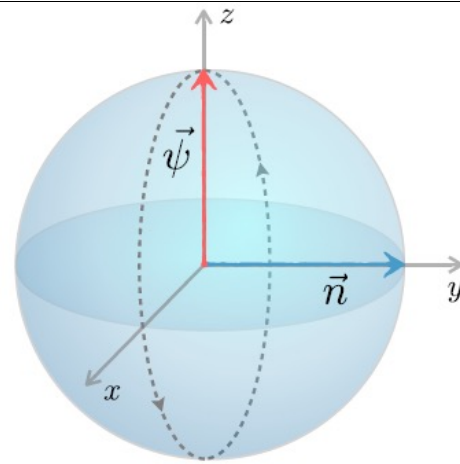
Figure 2b. A simple form of dynamics regarding Prob_A(t) (projection along the z-axis), where H = \sigma_y . Probability Prob_A(t) oscillates between 0 and 1.
