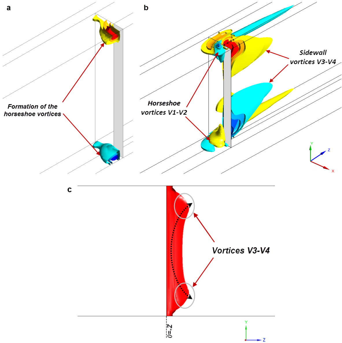
Fig. 8. Iso-surfaces of (a) the \omega_x and (b) the \omega_z vorticity ( Re_1=519 ). Three pairs of surfaces of equal magnitude ( \omega_x=100-75-50 \text{ s}^{-1} , \omega_z=50 - 25 -12.5 \text{ s}^{-1} ) and opposite sign are presented (red-maximum vorticity, blue-minimum vorticity). (c) Iso-surface of the total vorticity |\omega|=200 \text{ s}^{-1} .
