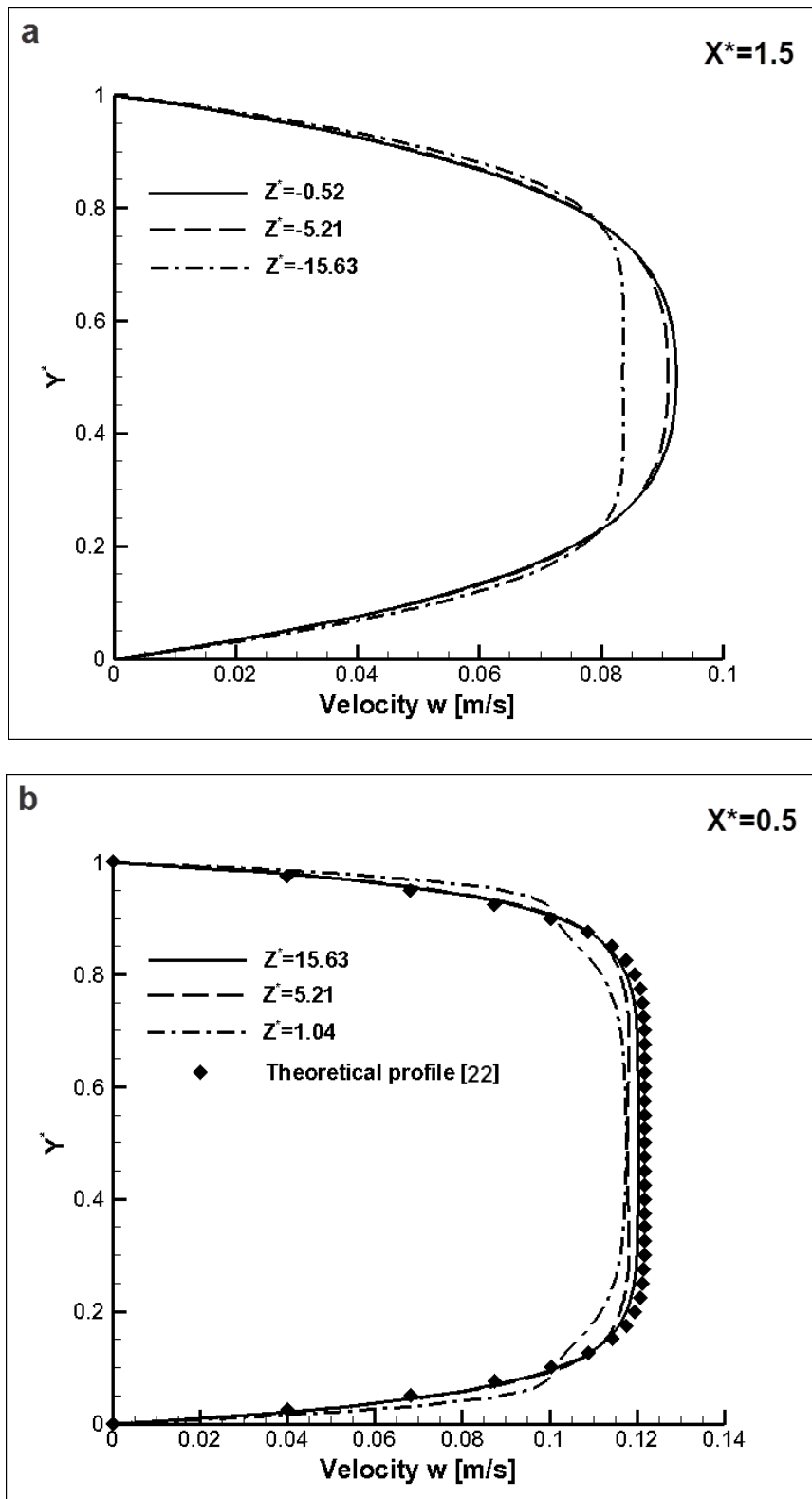
Fig. 5. Vertical profiles of w -velocity at the (a) first ( Z^* < 0 ) and (b) second section ( Z^* > 0 ) of the unit cell.
