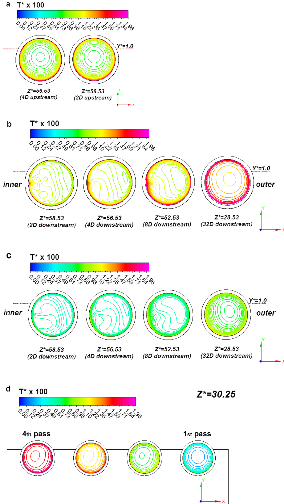
Figure 11. Temperature contour plots in the fluid region (solid top surface shown at Y^*=1 ): (a) upstream tube section of the two-pass configuration, (b) downstream tube section of the two-pass configuration, (c) downstream tube section of the four-pass configuration (second passage), (d) at the passages of the four-pass configuration.
