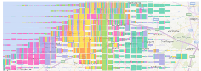
Figure 5: A tile map, but rather than temporal signatures inside each grid, stacked barcharts of the relative occupancy (width) and absolute occupancy (height) are embedded, showing the spatial occupancy of individuals (hue).
