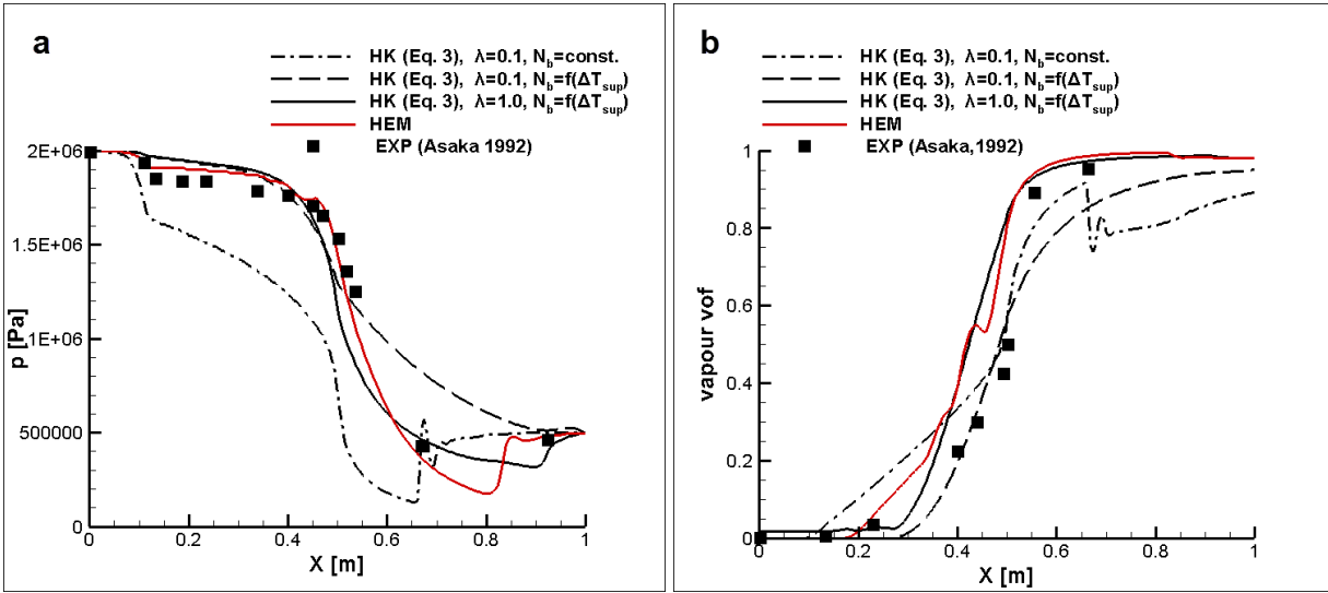
Figure 6. “Moby Dick” nozzle-Effect of the nucleation-site density distribution on the produced results: (a) pressure and (b) vapour volume fraction distribution.
