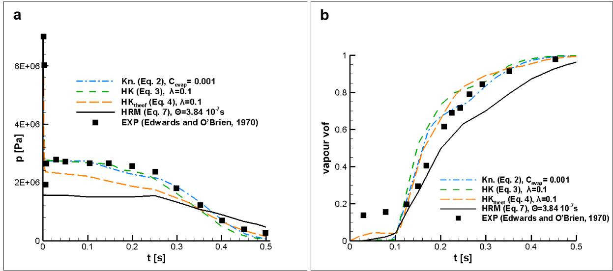
Figure 12. “Edwards’ pipe”-Comparison of the numerical predictions to experimental data: (a) pressure at the pipe (left) outer wall, (b) vapour volume fraction at the pipe mid-section.
