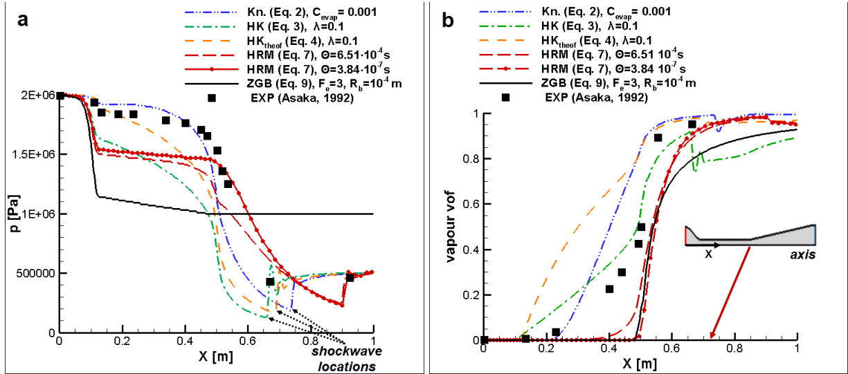
Figure 5. “Moby Dick” nozzle-Comparison of the numerical predictions to available experimental data: (a) Pressure and (b) vapour volume fraction at the axis along the nozzle length.
