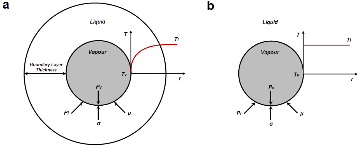
Figure 2. Schematic of growing bubble and surrounding liquid for thermodynamic (a) equilibrium and (b) non-equilibrium conditions.
