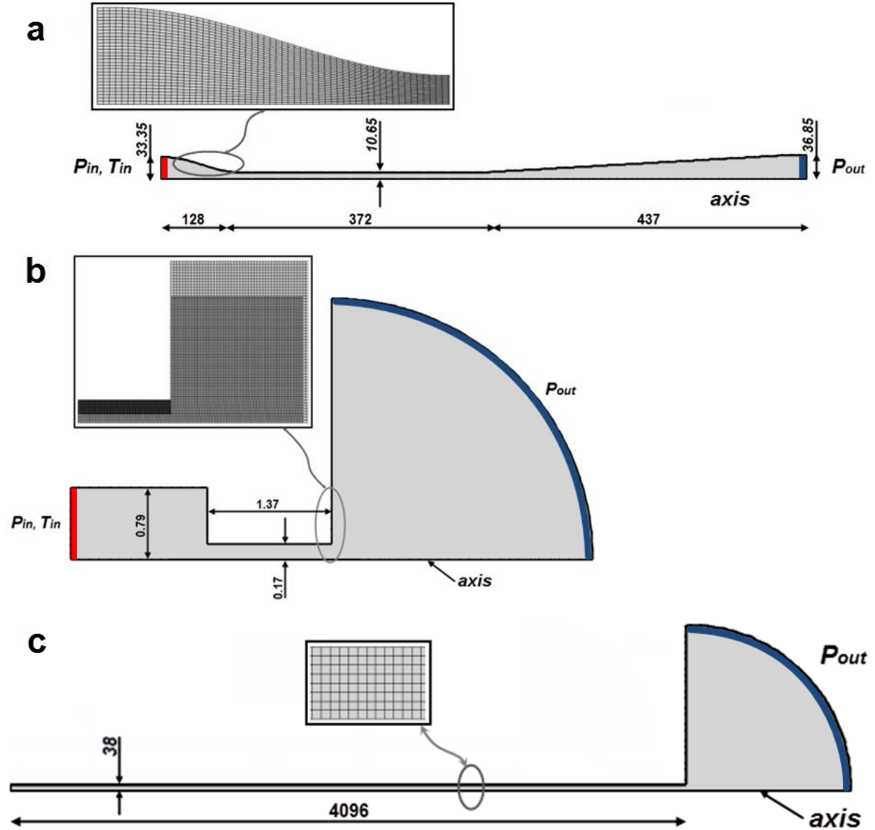
Figure 1. Computational domain and grid topology (all dimensions in mm): (a) "Moby Dick" nozzle, (b) "Reitz" nozzle, (c) "Edwards' pipe".
