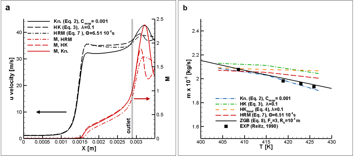
Figure 9. “Reitz” nozzle: (a) Velocity and Mach number distributions at the nozzle axis and (b) mass-flow rate at the nozzle inlet.
