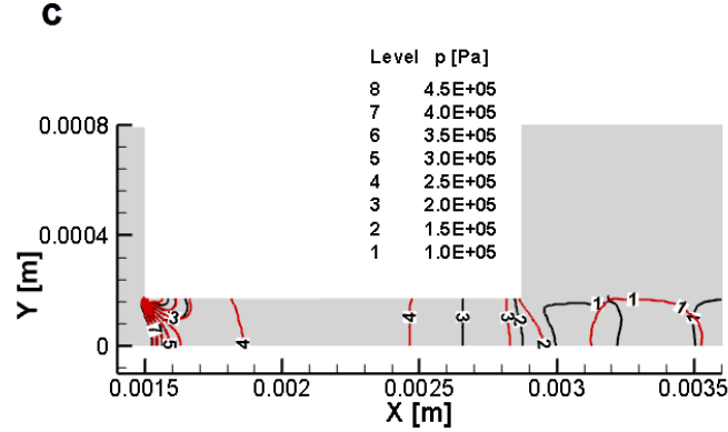
Figure 8. “Reitz” nozzle-Contour plots of the pressure field for T=427K : (a) Hertz-Knudsen, Eq. (3) ( \lambda=0.1 ), (b) HRM, Eq. (7) ( \Theta=6.51 \cdot 10^{-4}s ) and (c) comparative contour plot with black and red lines corresponding to the predictions of HK and HRM, respectively.
