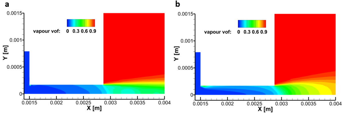
Figure 7. “Reitz” nozzle-Contour plots of the phase field for T=427K : (a) Hertz-Knudsen, Eq. (3) ( \lambda=0.1 ), (b) HRM, Eq. (7) ( \Theta=6.51 \cdot 10^{-4}s ).
