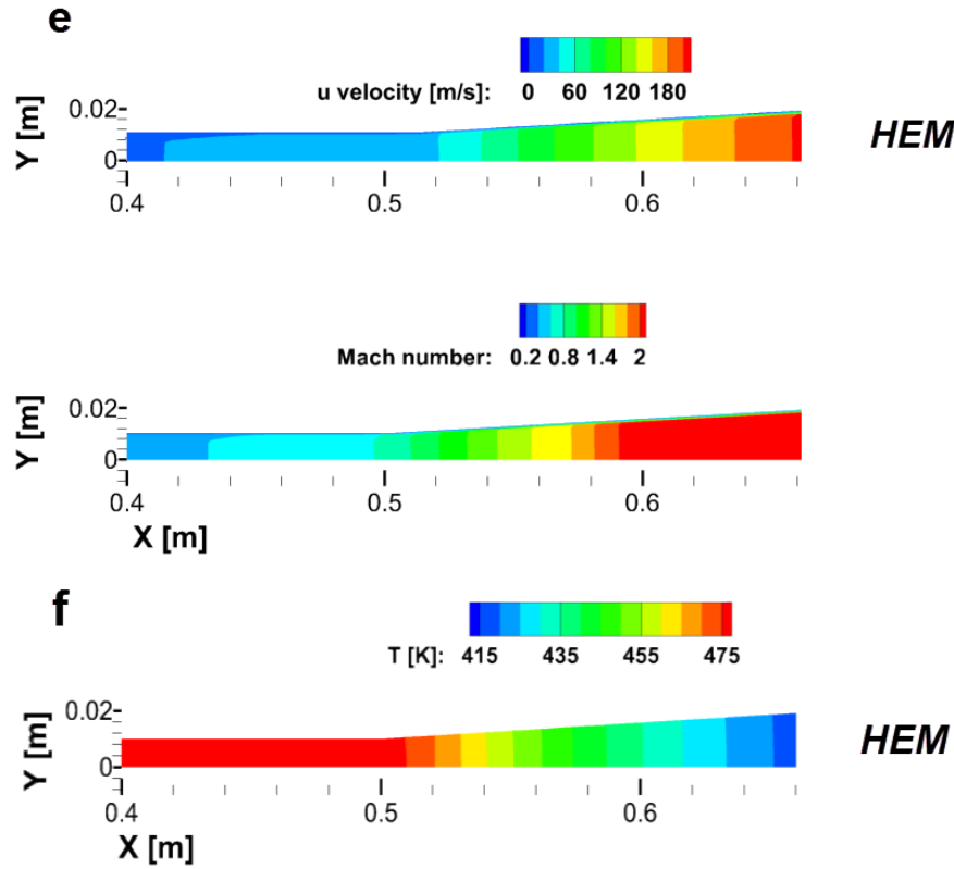
Figure 4. “Moby Dick” nozzle-Contour plots of (a, d) the pressure, (b, e) velocity and (c, f) temperature fields at the throttle region, as predicted using Hertz-Knudsen Eq. (3) for \lambda=0.1 (a-c) and HEM (d-f).
