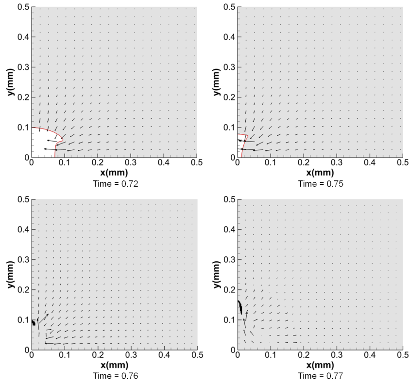
Figure 15: Depiction of the supercritical (black), vapour (white) and liquid (grey) regions, combined with velocity vectors for d=-140\ \mu\text{m} . Time has been non-dimensionalized with Rayleigh collapse time \tau=2.88\ \mu\text{s} .
