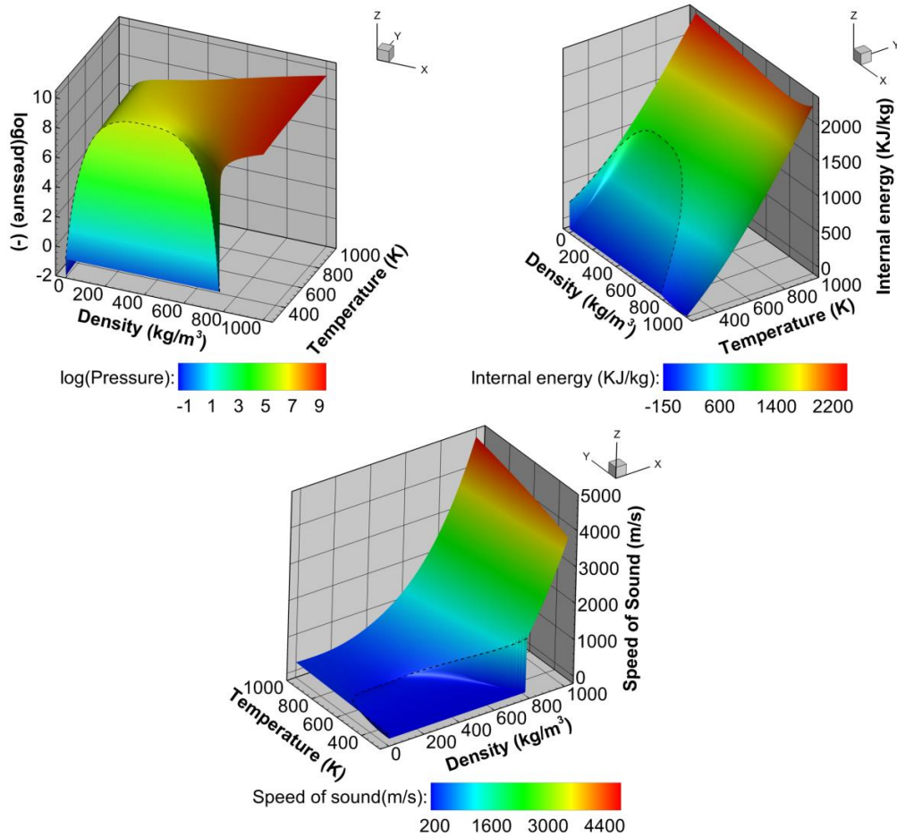
318 Figure 2: Three dimensional phase diagrams for the n-Dodecane, where the dashed line is the 319 saturation line. The properties have been derived from the Helmholtz energy EoS. 320
