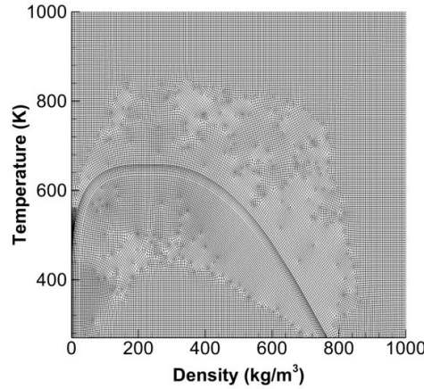
314 Figure 1: Unstructured thermodynamic grid of 40,000 finite elements, refined near the saturation line.
