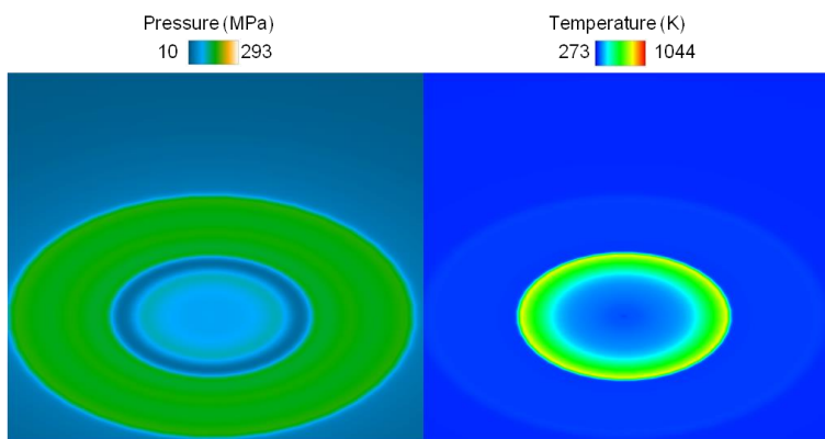
Figure 10: Wall pressure (left) and temperature (right) combined with density iso-surfaces of 380 \text{ kg/m}^3 during the vapour bubble collapse for d=140 \text{ μm} . Time has been non-dimensionalized with Rayleigh collapse time \tau=2.88 \text{ μs} .
