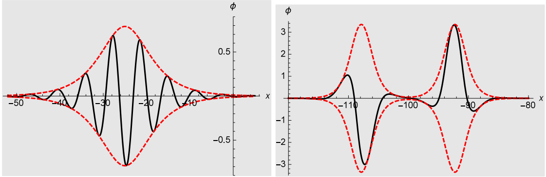
Figure 5: One-breather solution surrounded by enveloping function \pm \phi_{\tilde{\alpha},1/\tilde{\alpha}}^{\text{env}} at t = 25 for \theta = 1/5 panel (a) and degenerate two-breather solution surrounded by enveloping function \pm \phi_{\tilde{\alpha},\tilde{\alpha},1/\tilde{\alpha},1/\tilde{\alpha}}^{\text{env}} at t = 100 for \theta = 4/3 panel (b).
