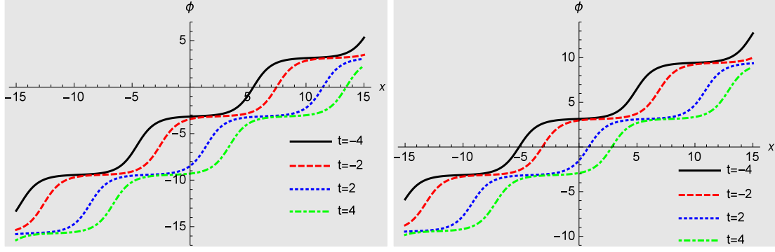
Figure 3: Sine-Gordon cnoidal kink solution \phi_{+,m,\beta}^{>(1)}(x,t) (panel a) and degenerate cnoidal kink solution \phi_{+,m,\beta\beta}^{c>}(x,t) (panel b) for spectral parameter \beta = 0.9 and m = 0.3 at different times.
