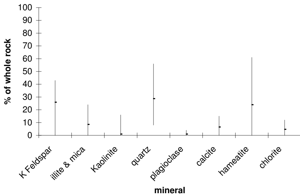
Figure 4.85 Abundances of minerals within the whole rock, remoulded soil
