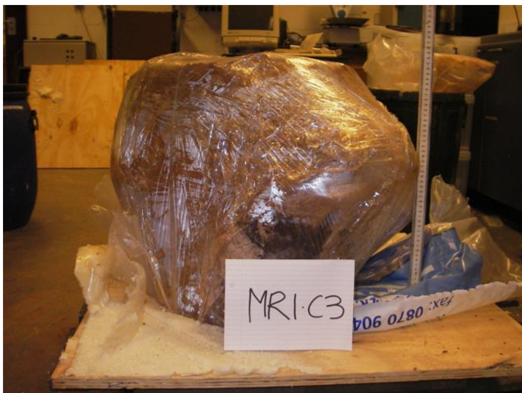
Figure 4.11 The section from pile MR1 819-1277mm below ground level
