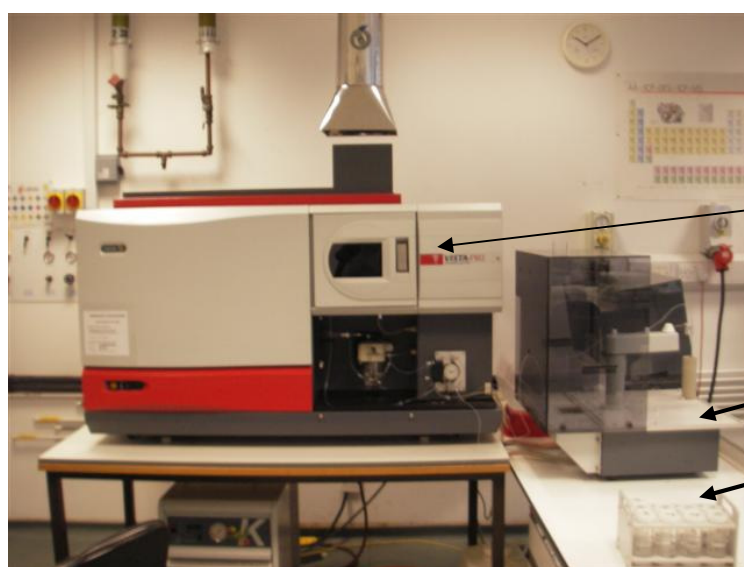
Figure 3.11 The ICP-AES
