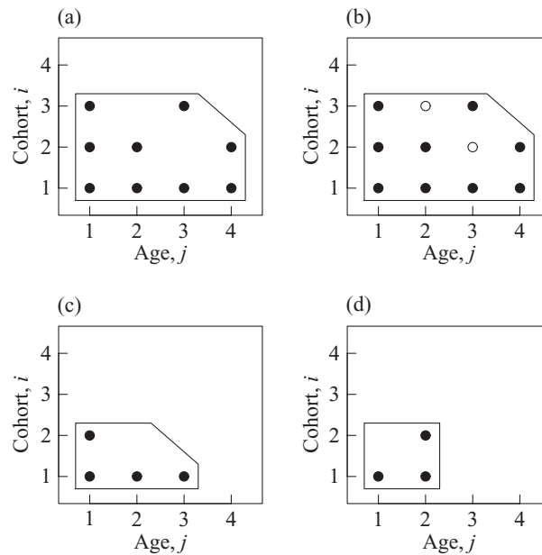
Fig. 2. Panel (a) shows an index set which is not a generalized trapezoid. This set is extended to a generalized trapezoid in panel (b). The sets in panels (a) and (b) have the same canonical parameter. Panels (c) and (d) show examples of sets which are not generalized trapezoids and for which the associated generalized trapezoid has a canonical parameter of larger dimension than the set itself.
