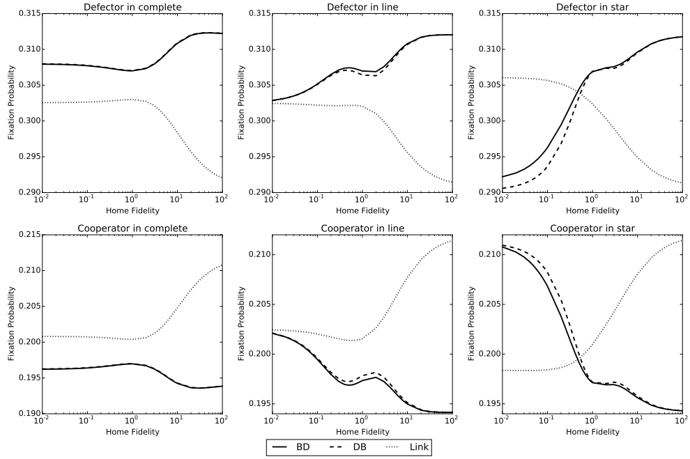
Figure 7.4: Comparison between BD, DB and Link dynamics for Def. 1. For the game r = 10 and v = 2 . The selection bias is x = 0.5 .
