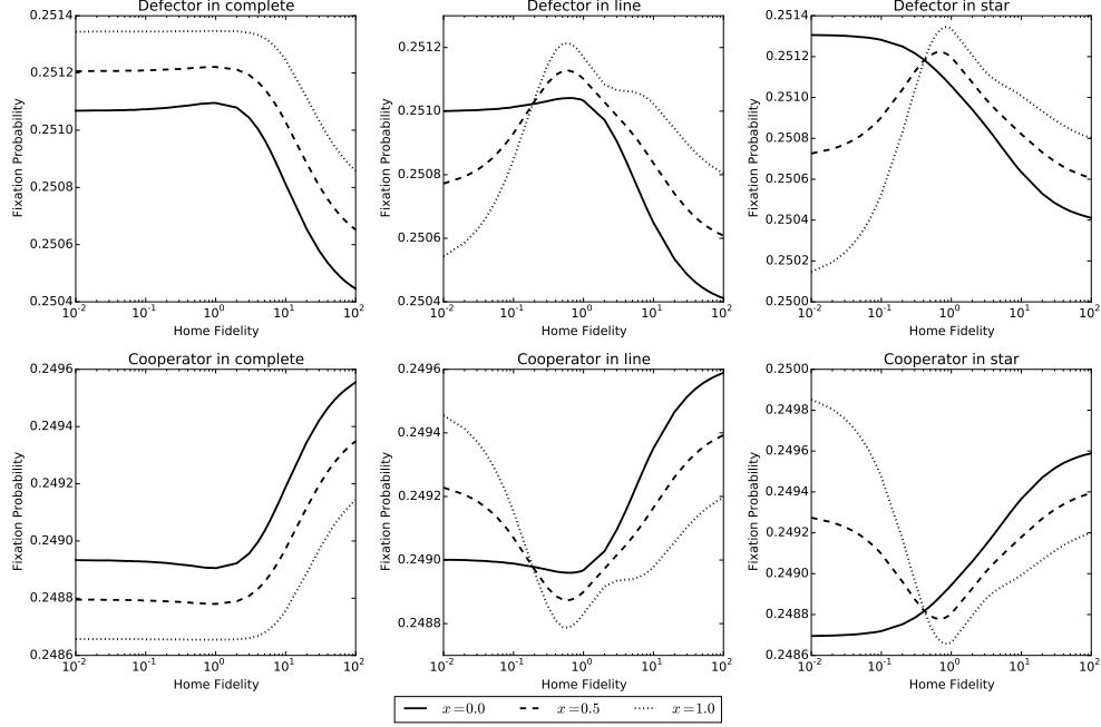
Figure 7.8: Comparing different values of the selection bias for BD Def. 3 dynamics. For the game r = 10 and v = 2 .
