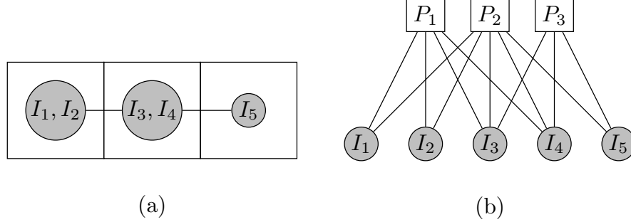
Figure 5.1: The territorial raider model with subpopulations. (a) Individuals that are members of subpopulation \mathcal{Q}_m live in place P_m but can visit neighbouring places. The territory of subpopulation \{I_1, I_2\} consists of places P_1 and P_2 , the territory of subpopulation \{I_3, I_4\} consists of places P_1, P_2 and P_3 , the territory of subpopulation \{I_5\} consists of P_2 and P_3 . (b) An alternative visualization as multiplayer interactions on a bi-partite graph where individuals and places are clearly separated.
