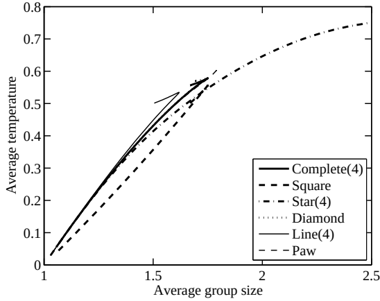
Figure 4.9: The mean temperature versus the mean group size for graphs with 4 vertices (as h varies from 0 to 100). For complete graphs, the line with 4 vertices and the diamond, i.e. the graphs where the mean temperature peaks at h \approx 1 , there is a spike in the correlation figure corresponding to the fact that the mean temperature and the mean group size increase (decrease) at different speeds as h < 1 (or h > 1 ). Note that Star(4) has the largest possible mean group size.
