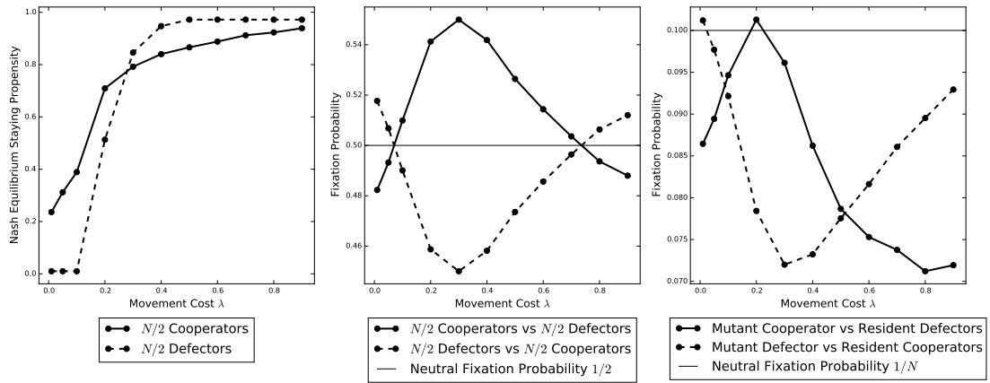
Figure 6.9: These plots show the effect of movement cost \lambda on the evolution of cooperation and are created using parameter set 1. The plot on the left shows the Nash equilibrium staying propensity \gamma for cooperators and \delta for defectors in a mixed population where there are N/2 individuals of each type. The plot in the centre shows the fixation probability of each type from the mixed state with N/2 individuals of each type. The plot on the right shows the fixation probability of a mutant cooperator C_\gamma (defector D_\delta ) in a population of N - 1 resident defectors D_\delta (cooperators C_\gamma ).
