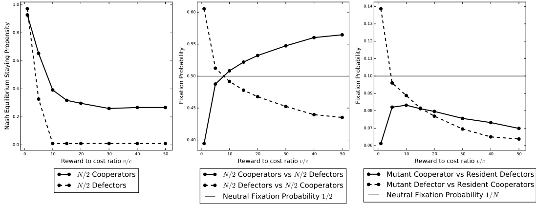
Figure 6.14: Plots created using parameter set 5. Plots are as in Figure 6.9 but \lambda is fixed and reward to cost ratio v/c varied such that c = 0.09 .
