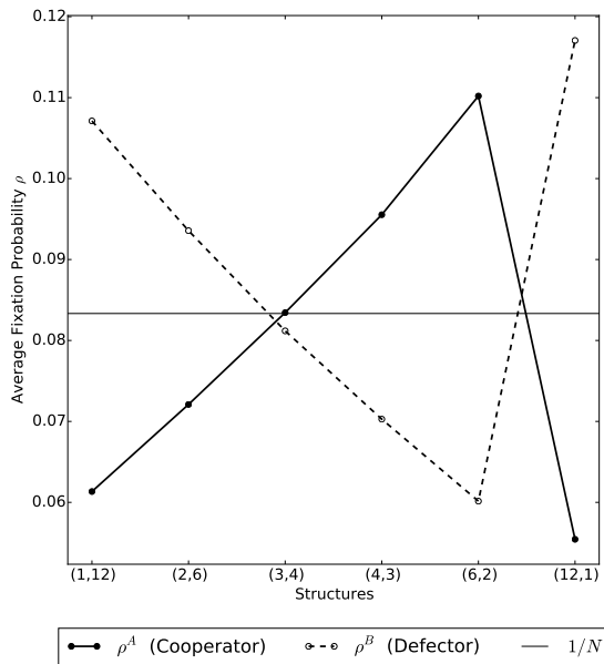
Figure 5.5: Comparing different population structures for the public goods game with various complete graphs for a population size of 12 where (1,12) means there is 1 subpopulation with 12 individuals, (2,6) means there are 2 subpopulations with 6 individuals and so on. The parameters are set to r = 30 and v = 10 , the dynamics used are DBB and for home fidelity h = 30 .
