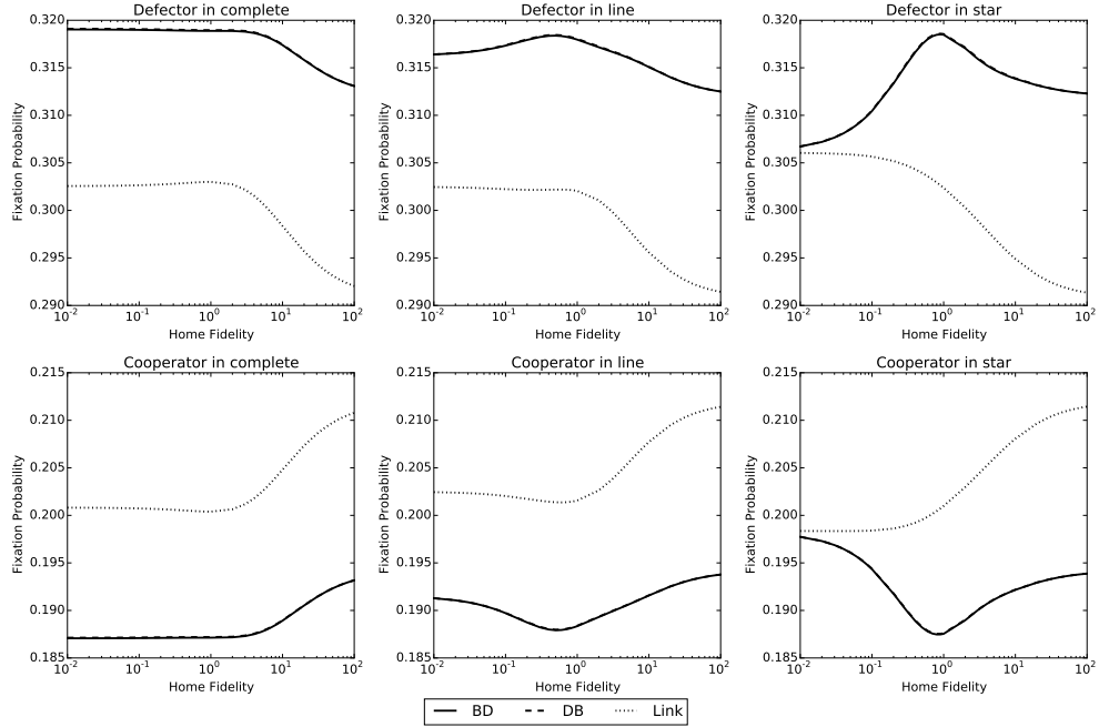
Figure 7.5: Comparison between BD, DB and Link dynamics for Def. 2. For the game r = 10 and v = 2 . The selection bias is x = 0.5 .
