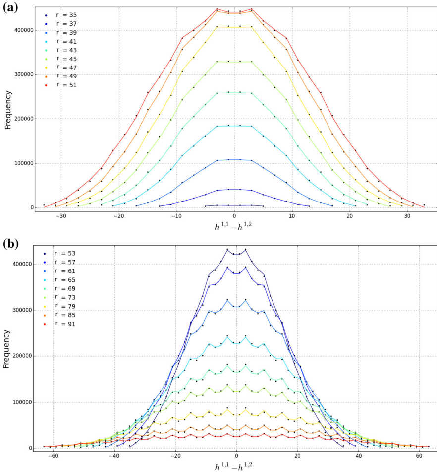
Fig. 5. Plots of frequency against h^{1,1} - h^{1,2} for various odd values of r . Each line represents a modified pseudo-Voigt profile based on the regression analysis for each curve. See Fig. 28a for a plot of all even curves. a Regression lines for all odd r valued curves, with r \in [35, 51] . b regression lines for few select odd r values, with r > 51
