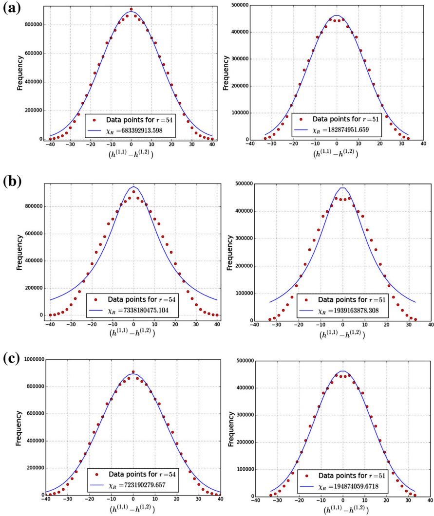
Fig. 25. For all models, the left hand graph is for r = 54 and the right is for r = 51 . The probability plot presents all the models together. All the above mentioned modeled are included to compare their resemblance with the actual data. The larger the p value the better the line y = x fits the data, implying the better the model is at describing the data. a Gaussian model. b Lorentzian (Cauchy) model. c Pearson7 model. d Breit–Wigner model. e Voigt model. f Pseudo-Voigt model. g The probability plot for r = 51 . h The probability plot for r = 54 .
