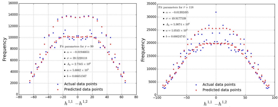
Fig. 7. These two plots serve two purposes. The first is to show how the modeled data should really look by using data points (red points) instead of the (perhaps misleading) lines (refer to Comment 1 below). The second purpose is to illustrate that as r becomes large (left plot has r = 99 , right plot has r = 118 ), the actual data points deviate more and more from the modeled data, implying that there is a missing function in the modified pseudo-Voigt model which would allow one to describe the data at much lower frequencies (color figure online)
