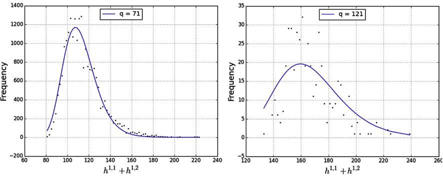
Fig. 35. Left figure is the fitted model (blue line) for a q value of 71 and right has a q value of 121. As the q -value increases, the scattering of the data points within h^{1,1} + h^{1,2} increases to the point where the model works no longer. For an example of how the model begins to break down at large q , see Fig. 15
