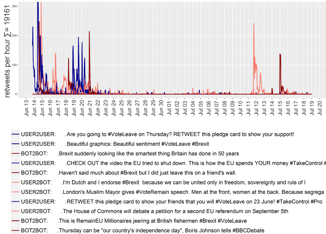
Figure 5: Large cascades ( S > 506 ) from user to user, bot to bot, and user to bot
