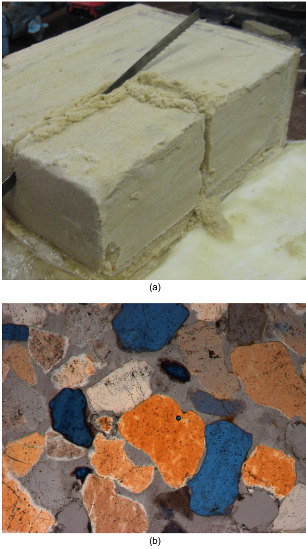
Fig. 5. Intact Reigate sand: (a) illustration of the block sample; (b) micrograph of a thin section under cross-polarised light showing the extended flat contacts between the grains (after Fonseca, 2011)
