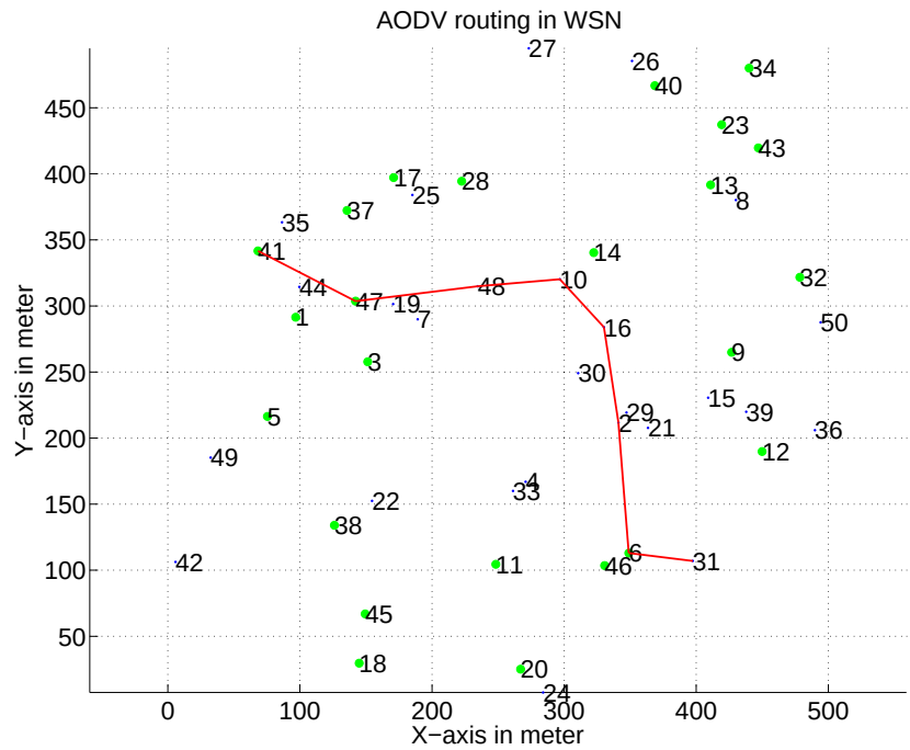
Fig. 3.3 A simple example: route Determined by AODV
