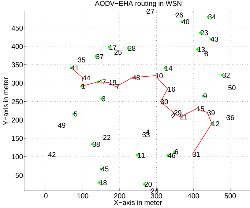
Fig. 3.5 A simple example: route determined by AODV-EHA
