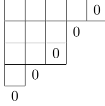
Young diagram of \lambda = (5, 3^2, 1) .
