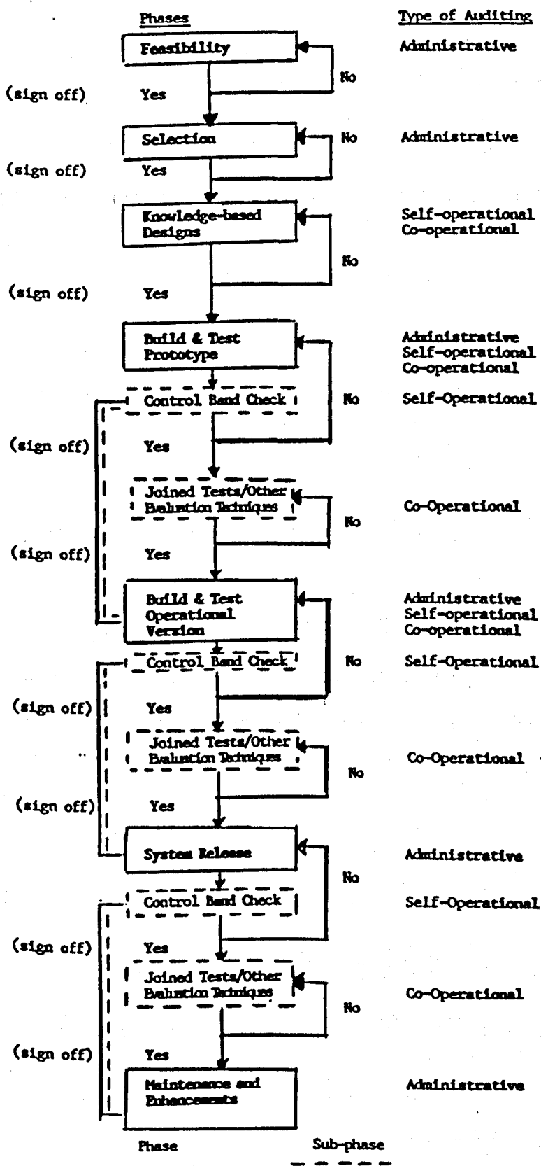
Fig:10: Modular Model - Auditing an Expert System Under Development
